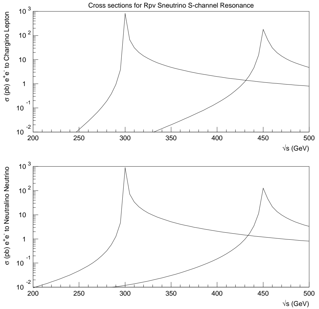
Figure 3: The parameters for this plot are the following: m_{\tilde{\nu}} = 300 and 450 GeV respectively; m_{\tilde{e}} = 1000 and 450 GeV; \tan\beta = 2 , \lambda = 0.1 , \mu = -200 , M_2 = 250.0 . In this case, all charginos and neutralinos are produced.
