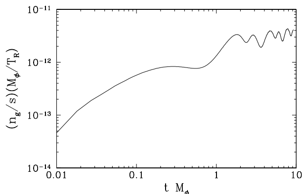
Figure 4: The ratio n_g/s as a function of time for \phi_0/M_{\text{P}} = 10^{-1} and for a quadratic superpotential.
