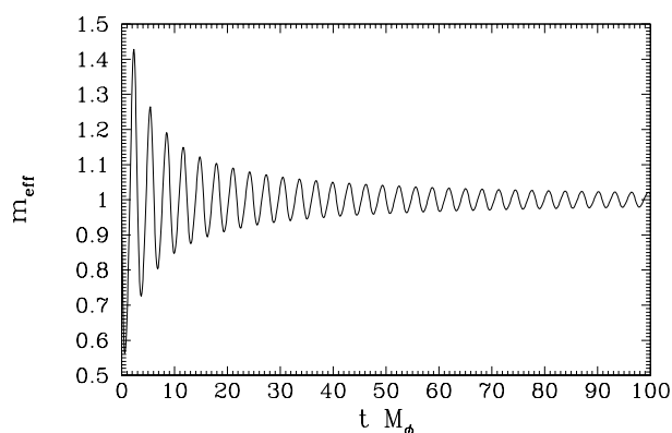
Figure 2: The evolution of the parameter m_{\text{eff}} in units of M_\phi as a function of time and for a quadratic superpotential. The initial condition is \phi_0/M_P = 10^{-1} .
