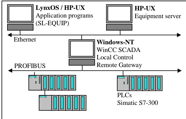
Figure 1: Hardware architecture.
