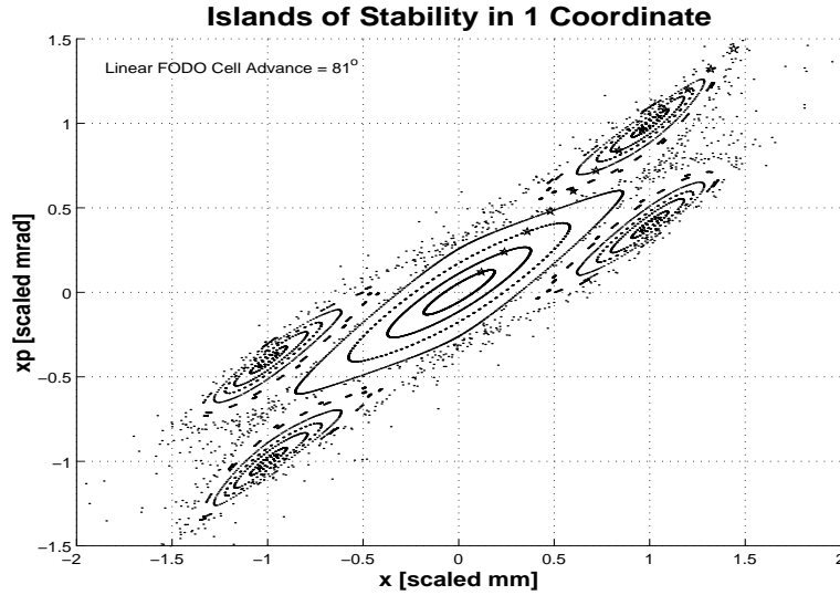
FIGURE 5. One coordinate only was used in this calculation without the cross coupling terms in x and y , and, therefore, islands of stability appeared. A FODO lattice with 81^\circ linear phase advance and 500 FODO cells, Quadrupoles and Octupoles, was used. The way this figure has to be interpreted is as a sequence of separate single particle motions. The particles are started in the diagonal of phase space, as indicated by the star symbols. They are plotted for each quadrupole. For the particles with a small amplitude in the center nothing happens. The Octupole fields are too weak to influence the motion and so these particles stay on their closed ellipse in phase space. For particles with larger amplitude the phase space gets deformed, and finally they get unstable (e.g., follow the particle with x=0.62 ). But then the system recovers, and particles are stable again; but not on closed ellipses, they hop from island to island. Figure 4 did show how the effective phase advance in the system changes; for the islands it should be assumed that this phase was close to, and passing through, 90^\circ . Particles even further out then quickly get lost (collimated).
