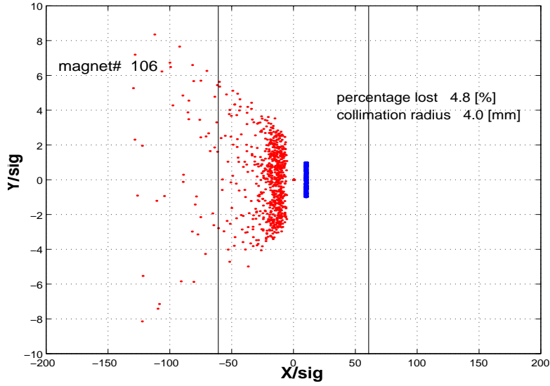
FIGURE 11. Same as Figure 10, for a 4 mm collimation radius. Note the large difference in penetration depth as compared to the case of a 3 mm collimation radius in Figure 10, indicative of the non-linear effects. Also note that the percentage loss is about the same.
