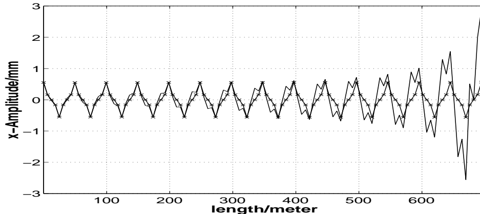
FIGURE 4. Although only one coordinate is shown here, this calculation was done for a realistic Octupole field with the required cross coupling terms in x and y . The single particle motion in the linear (Quadrupoles only) and non-linear (Quadrupoles and Octupoles) case are compared. The starting value was x = 600 \mu\text{m} (corresponding to 9 \sigma in the NLC main linac) and x' = 0 . The positions of the Quadrupoles is indicated with x 's in the linear case. This curve shows the very regular even pattern of a constant 90^\circ FODO lattice. The added kicks of the Octupoles have the effect of changing the effective phase advance to higher values. The amplitude changes, slowly at first, then rapidly, until the particle gets lost at about 3 mm of amplitude. Note that this combined phase advance depends strongly on the position in x, y space, making predictions of when a particle will get lost close to impossible in general. This example was calculated with the standard NLC main linac lattice cell length of 12.5 m and Octupoles with a 3kG pole tip field at a pole tip radius of 5 mm ( k_3 = 43300 \text{m}^{-3} in MAD notation).
