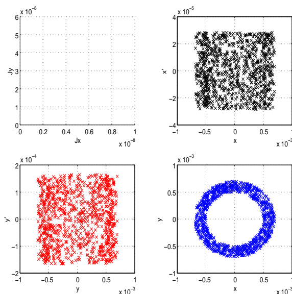
FIGURE 15. Patterns of Halo particles created from a concentric Halo Ring in real space, combined with random x' and y' . Subfigure a is empty but carried along to allow direct comparison with action variable plots later. Subfigures b and c show the particles used in the x, x' and y, y' space. Subfigure d finally shows the Halo ring, from which the phase space distributions are derived, in real space. Since the phases are randomly chosen, the phase space distributions are filled in. The next Figure shows that the magnitude of the distributions are the same, but that with action variables the phase space envelope is elliptic (as it should be) and not a rectangle as here.
