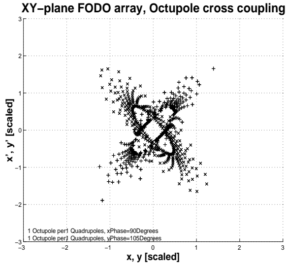
FIGURE 9. Phase space plot of one particle in x and y phase space. The particle goes through a 100 cell FODO lattice with a phase advance of 90^\circ and 105^\circ in x (x's) and y (+s), respectively. This simulation was performed with a full coupled matrix multiplication. The figure has to be interpreted as the (one) particle initially being on its unperturbed phase ellipse(s), then slowly spiraling out under the relentless kicks of the Octupoles, until it is abruptly lost.
