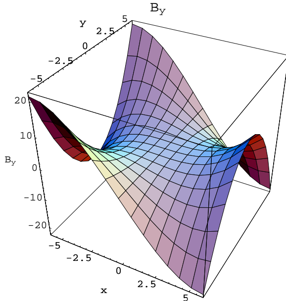
FIGURE 7. The 3-dimensional display of the B_y -field of the Octupole field of Figure 6. The B_x -field looks the same, with x and y rotated. The figure shows that for large amplitudes the cross-coupling terms, off the x and y -axis, dominate the on-axis fields.
