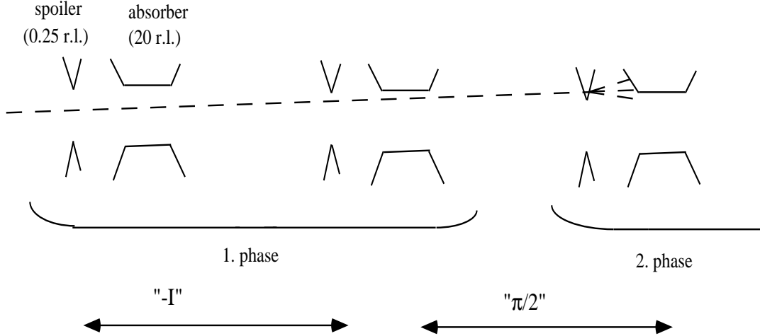
FIGURE 2. Schematic of a conventional collimation system taken from [5], consisting of a series of spoilers and absorbers which collimates in two planes and two lattice phase advances. The size of the spoilers and absorbers is approximately 1/4 and 20 radiation lengths (r.l.), respectively. A beam coming from the left hits first a spoiler, where its size is enlarged, before it interacts with an absorber.
