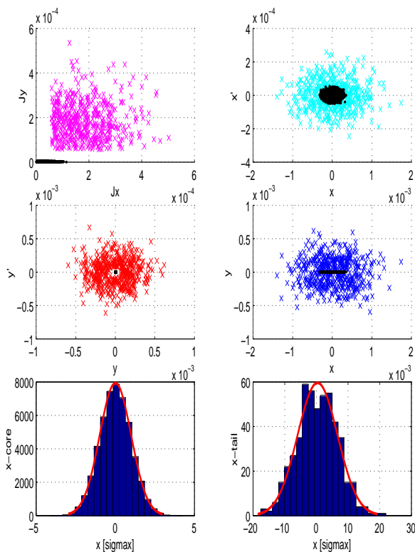
FIGURE 19. Patterns of core (50,000) and Halo particles (500) created with the method explained above, for the parameters of the pre-linac case. Subfigures a to d correspond to Figure 17. Subfigure a shows the flat "core" in the lower left corner and the Halo in J_x + J_y space above it. Note again, as described in the text, that the Halo corresponds to an exponential distribution starting at (the equivalent of) 3.29 \sigma in both x and y , and that the width of the Halo distribution is 10 times the width of the core. Subfigures b and c show the relation of cores and Halos in the x, x' and y, y' space. Subfigure d shows the equivalent of Halo Ring in real space around the flat core beam. Since the amplitudes and phases are randomly chosen, the "rings" are filled in, as before. Since the "Halo" is constructed to be symmetric in space, but the core beam is flat, the Halo phase space touches the x -core in b, but stays well clear of the y -core distribution in c. Subfigure e shows a histogram of the core in transverse x -coordinate, and f finally shows the tail in x . As expected the core has a width of 1 \sigma and the tail of 10 \sigma . Note further, that the tail as a projection of a circular distribution onto the x -axis seemingly has a dimple in the middle, as it should.
