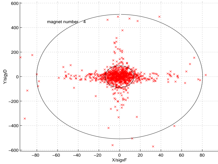
FIGURE 25. This Figure shows the real space distribution in the 1 st magnet in the 3 rd FODO cell, a horizontally focusing Quadrupole. Particles are spread out horizontally and vertically and are being collimated.
