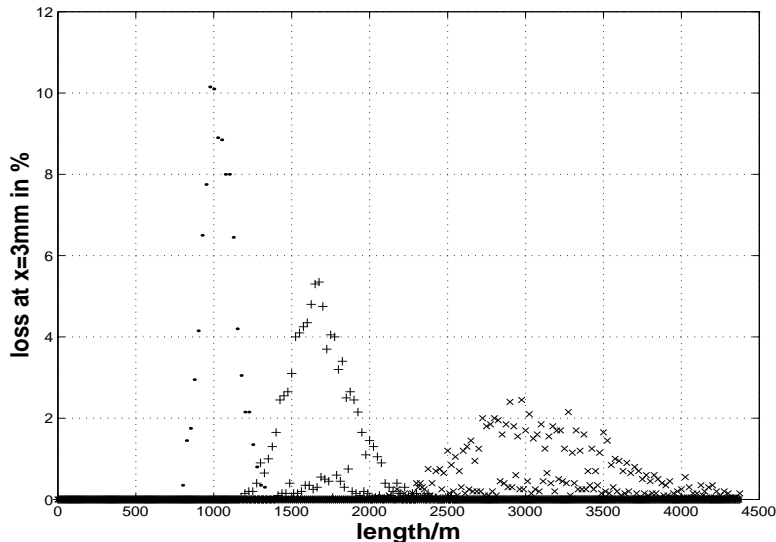
FIGURE 13. Pattern of loss of an errant beam along the linac with a 3 mm radius absorber. The 3 distributions correspond to an initial offset of 25, 20, and 15 sigma, as shown from left to right. As will be shown in the treatment of the linac case below, the strength of the Octupoles has to be sufficiently high to prevent new background to be created from tails close to the core. This example has a strength k_3 = 4320m^{-3} . Here, beams with off-sets larger than about 20 \sigma will be lost in too small a region.
