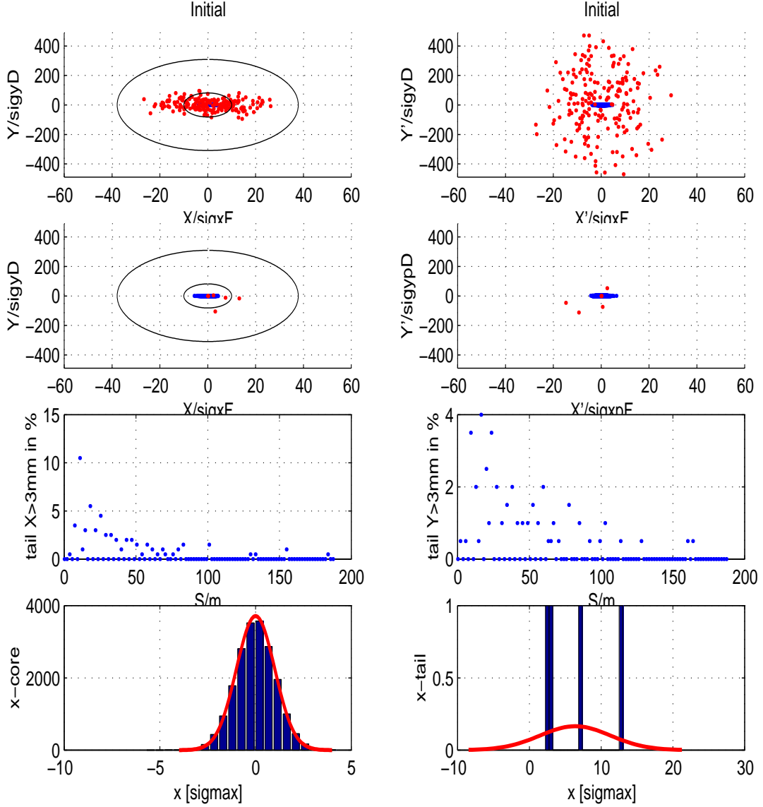
FIGURE 23. This Figure for the pre-linac is different from the ones shown before, in as much as it shows the initial distribution in x-y and x'-y' space, (subfigure a and b), the same parameters after collimation (subfigures c and d), the loss process along the accelerator in both x and y (subfigures e and f), and the x-core and x-tail after collimation (subfigures g and h). The core (20000) and Halo particles (200) were created with the total tail method explained above. The circles in subfigures a and c are the beam stay clear (inner circle, here a 10\sigma radius) and the collimation radius used (3 mm radius, outer circle). As explained earlier in the text the main reason for doing the simulation with a total tail approach, rather than the Halo Ring approach, is to test graphically if there is bleeding from the core into the tails. None did. One also has to test if particles get beyond the BSC without being removed beyond 3 mm. 2 out of 200 (2%) did. Note again, as described in the text, that the Halo corresponds to an exponential distribution in J-space starting at (the equivalent of) 3.29\sigma in both x and y, and that the width of the Halo distribution is 10 times the width of the core.
