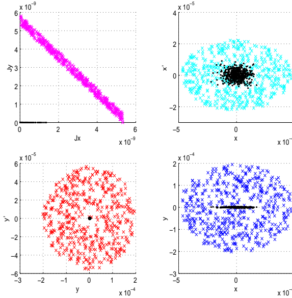
FIGURE 17. Patterns of core and Halo particles created with random phases and constant sum of amplitudes. Subfigure a shows the flat "core" in the lower left corner. The J_x + J_y = \text{const} particle stripe corresponds to the Halo Rings explained before. Corresponding to the increase in radius of a Halo ring is the movement of the stripe diagonally to the upper right, as "const" is increased. Subfigures b and c show the relation of cores and Halos in the x, x' and y, y' space. Subfigure d shows the equivalent of Halo Rings in real space. Since both amplitudes and phases are randomly chosen, the "rings" are filled in (and are no longer rings). Since the "Halo" is constructed to be symmetric in space, but the core beam is flat, the design Halo to be collimated touches the x -core, but stays well clear of the y -core distribution.
