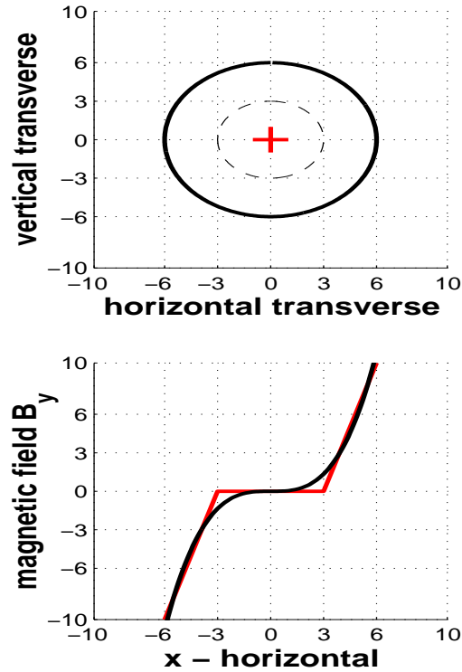
FIGURE 1. The top part shows the conceptual division of an accelerator in two concentric parts, with their separate lattices. Since this is physically not possible, ideally magnetic elements have to be found which are zero in the center and linear in the Halo region (light curve in the lower part). Maxwell's equations make this also impossible, so a compromise, here an Octupole field, is shown (dark curve in the lower part). But theoretically, see below, higher order multipoles have to be even better, although physically more difficult to build. It should strongly be emphasized that non-linear RF fields also should be considered.
