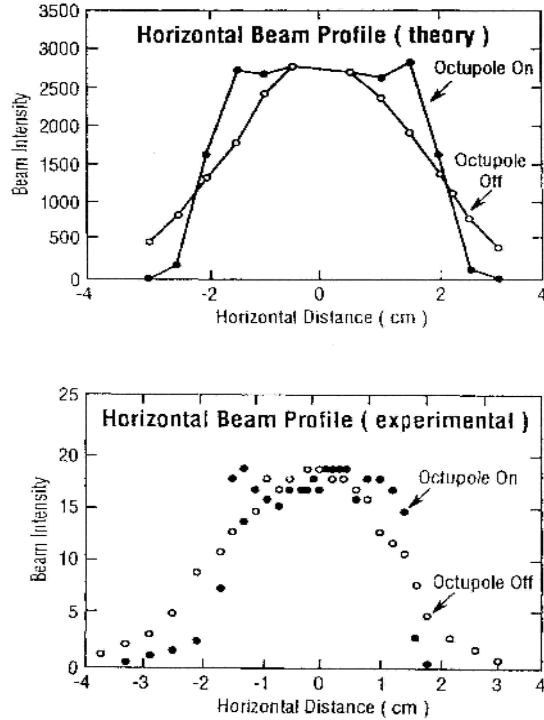
FIGURE 27. Comparison between theory and experiment for folding in the tails to illuminate a target uniformly from Reference [10].
