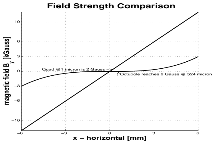
FIGURE 8. The magnetic field a standard collider Quadrupole reaches at 1 \mu\text{m} is about 2 Gauss, an appropriate Octupole reaches these 2 Gauss at a much larger off-set: 500 \mu\text{m} .
