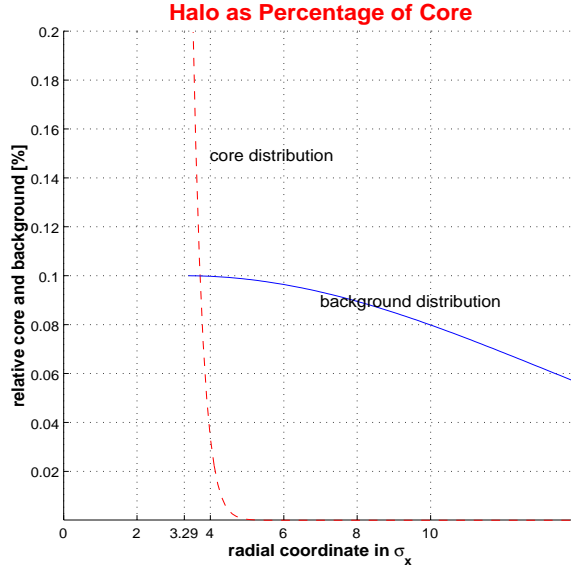
FIGURE 18. The construction of the SLC/SLD-like Halo attaches a radially symmetric 1% Halo to the 100% core at a point where the core is 0.1% of its maximum value.
