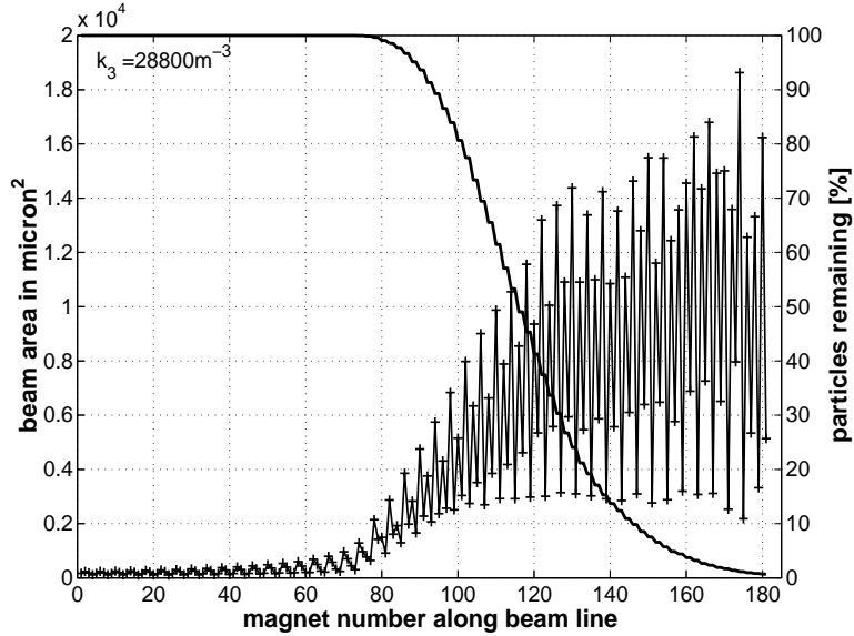
FIGURE 14. Development of the size, and the corresponding loss, of an errant beam along the linac with a 3 mm collimation radius as defined above. This example has been calculated with an Octupole strength of k_3 = 28800\text{m}^{-3} . The smooth curve describes the beam percentage still remaining, and the ragged curve the corresponding beam area in \mu\text{m}^2 . One realizes from Figures 10 and 11 that most of the size enlargement happens in the horizontal. So in principle the beam has the shape of a horizontal knife slicing into material it encounters, however, now the average angle \langle x' \rangle becomes important, spreading the interaction area over a large distance.
