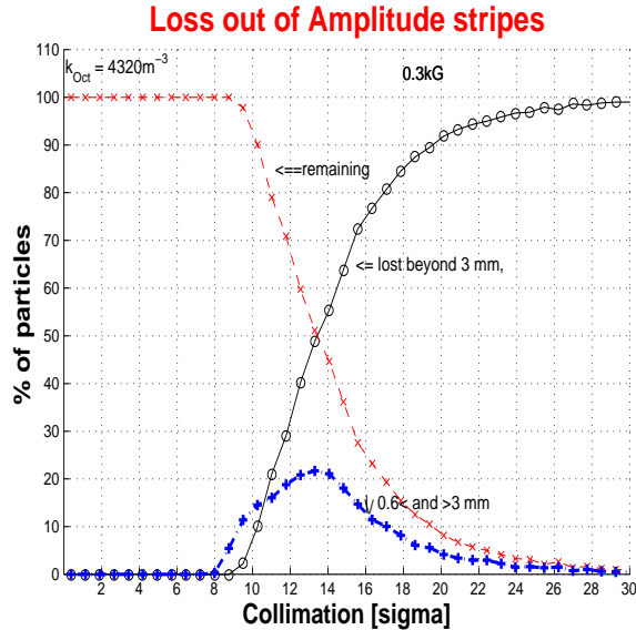
FIGURE 22. This main linac figure for k_3 = 4320m^{-3} , as the two figures before, shows three curves. It is important to realize is here that only particles outside of 8\sigma are being collimated, a \sigma -space where there are no core-like densities.
