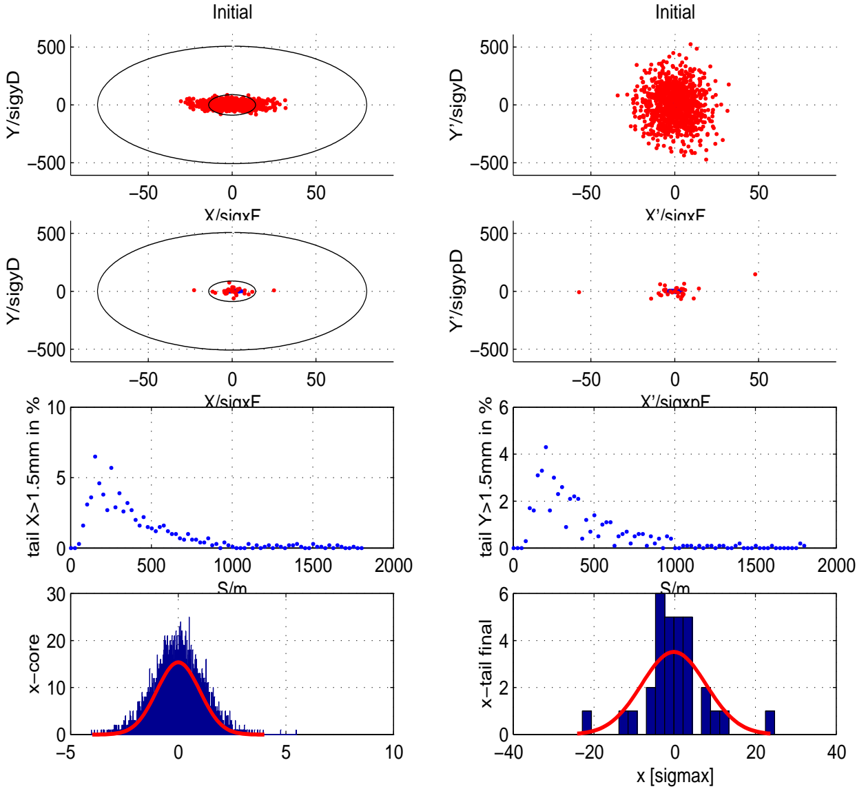
FIGURE 24. This Figure for the post-linac collimation is made with the same template as Figure 23, so the general explanations in the previous Figure apply. The core and Halo particles were created with the method explained above, but the number of core and tail particles was changed to 10000 and 1000, respectively, for better statistics with the tail simulations. The other parameters chosen were 36 FODO cells of 50 m length. The circles in subfigures a and c are the beam stay clear (0.25 mm, inner circle) and the collimation radius used (here a 1.5 mm radius, outer circle). Note again, as described in the text, that the Halo corresponds to an exponential distribution in J-space starting at (the equivalent of) 3.29 \sigma (equivalent to 0.1% in a Gaussian distribution) in both x and y, and that the width of the Halo distribution is 10 times the width of the core. The collimation of the post-linac beam is the most challenging for several reasons. The beams are small, the energy is high, and the space is not free, as in the other systems treated before.
