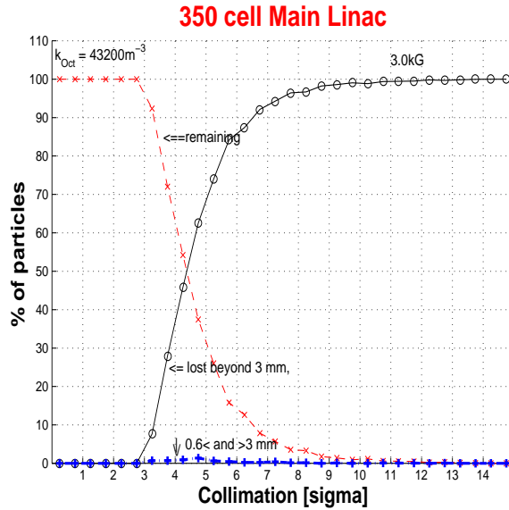
FIGURE 20. This main linac figure, as the next two, shows three curves. The calculations were done with a granularity of 0.5 \sigma in x , that means distributions were constructed which correspond to amplitude sums (rings) centered at 0.25, 0.75, 1.25 \sigma etc., with a width of 0.5 \sigma each. These distributions of particles then were passed through the modified FODO lattice. The rising curve shows the percentage of particles lost out of each stripe (=ring). A very important aspect is that most the particles "lost" out of the "ring" were brought to a position beyond 3 mm, the "collimation radius". The ones which were not lost are shown on the second, the bottom, curve. These latter particles are potentially dangerous, because they could hit material in the BDS and produce background. The third curve, of remaining particles, falling from 100% at the left, finally shows another important aspect: the inner 3 \sigma of the distribution are not touched. Even with 10^6 particles in the area between 2.5 and 3.0\sigma , not a single one was removed from this area. This is even more pronounced in the next two Figures, which show results with weaker Octupoles.
