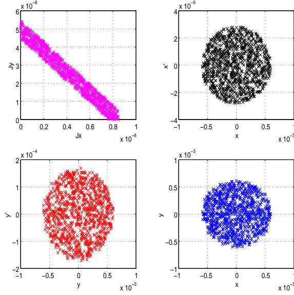
FIGURE 16. Patterns of Halo particles created with random phases and constant sum of amplitudes, designed to replace the "ring" of Figure 15. The J_x + J_y = \text{const} particle stripe in subfigure a corresponds to the Halo Ring explained before. Corresponding to the increase in radius of a Halo Ring would be the movement of the stripe diagonally to the upper right, as "const" is increased. Subfigures b and c show the relation of cores and Halos in the x, x' and y, y' space. Subfigure d finally shows the equivalent of Halo Ring in real space. Since both amplitudes and phases are randomly chosen, the x, y distribution is also filled in, and no longer a ring.
