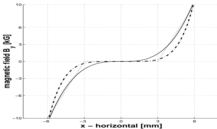
FIGURE 6. Comparison between the B-fields of an ideal magnetic element which leaves the center of the beam alone and influences only the tails (dotted curve), with actually buildable elements which will follow Maxwell's equations, here an Octupole (solid curve) and a Dodecapole (dash-dotted). For comparison the curves were normalized to reach 10 kG at 6 mm. They clearly show the theoretical advantage of a 12-pole.
