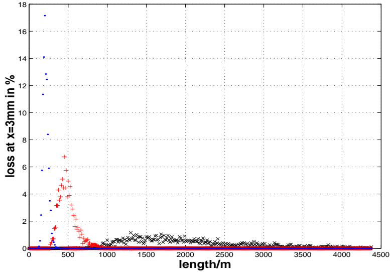
FIGURE 12. Pattern of loss of an errant beam along the linac with an Octupole strength of k_3 = 43200m^{-3} and a 3 mm radius absorber. The 3 distributions correspond to an initial offset of 15, 10, and 5 sigma, as shown from left to right. As will be shown in the treatment of the linac case below, the strength of the Octupoles has to be sufficiently high to prevent new background beyond the beam stay clear, but within the collimation radius, to be created from tails close to the core. But is has to be sufficiently weak to not transport particles from the core into the tails. Therefore, beams with off-sets larger than about 10 \sigma will have too large a loss in too small a length of linac and do damage independent of the enlarged size. Beams with an off-set larger than 10 \sigma , therefore, have to be prevented by other means.
