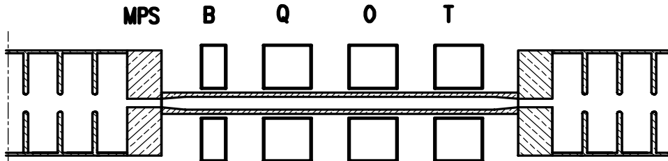
FIGURE 3. Schematic of the collimation assembly proposed: a circular copper pipe between acceleration sections, captured in the quadrupoles and Octupoles will suffice even for collimation of errant beams. The inner diameter of the collimator is thought to be 6mm, the outer diameter (OD) 10-13mm, depending on the pole tip radii of the magnetic elements. The pipe is tapered to match the aperture of the Machine Protection end-plugs (MPS) of the acceleration structures. The beam comes from the left, the copper pipe is captured in sequence by a BPM (B), a Quadrupole (Q), an Octupole (O), and finally a Tantalum block (T), if the latter is required at higher energies.
