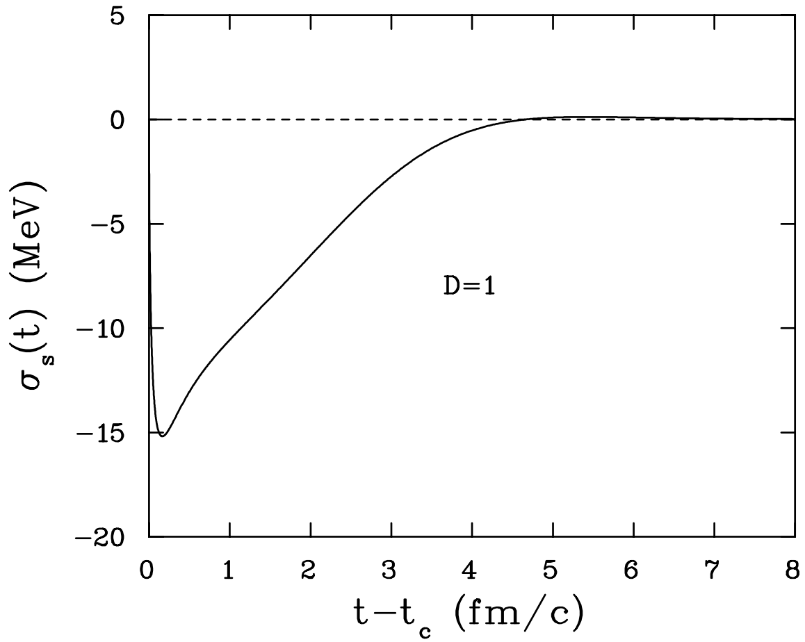
Figure 2: The temporal evolution of the deviation of the scalar condensate from its equilibrium value v in units of MeV for a one dimensional expansion of hot matter produced in a high energy nuclear collision.
