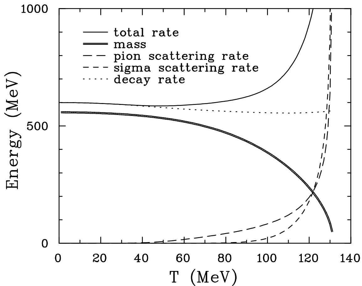
Figure 1: The sigma mass and the decay and scattering contributions to the width of the sigma meson as functions of temperature from 0 to T_c .
