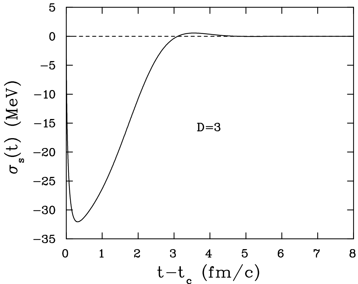
Figure 3: The temporal evolution of the deviation of the scalar condensate from its equilibrium value v in units of MeV for a three dimensional expansion of hot matter produced in a high energy nuclear collision.
