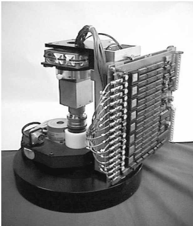
Figure 2: Fast Beam Profile Monitor
