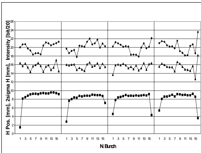
Figure 5: Evolution of first ions batch during the timing tuning of the CPS extraction kicker.
