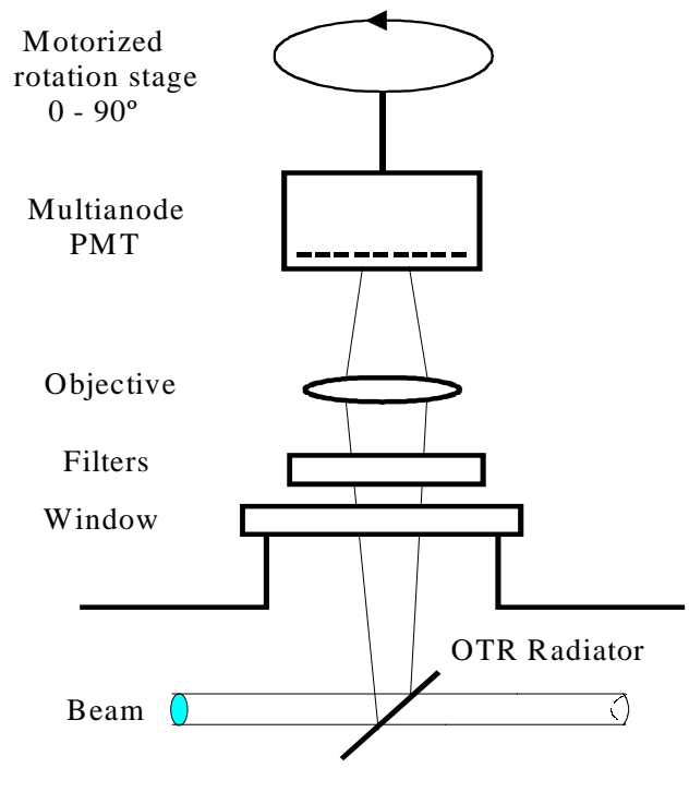
Figure 1: Schematic view of the monitor set-up
