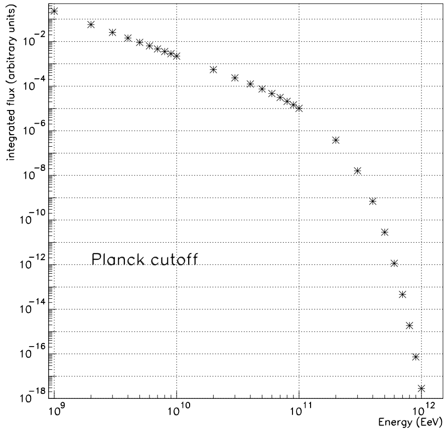
Figure 1: Planck cutoff effect on the integrated primary spectrum
