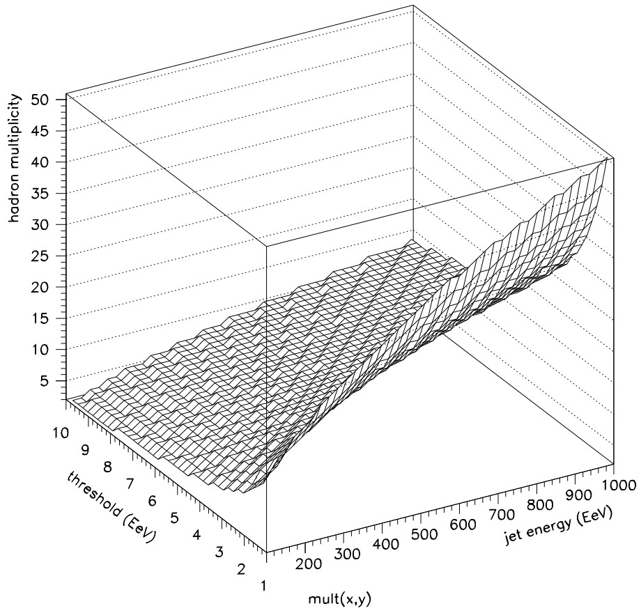
Figure 2: Hadron multiplicity as a function of the detection threshold and of the jet energy
