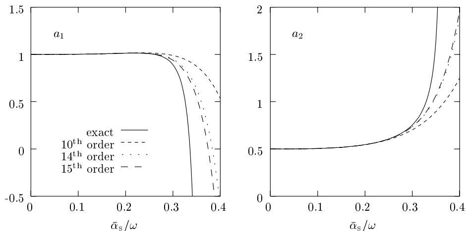
Figure 1: Coefficients in the mean jet multiplicity \bar{r}_\omega as functions of \bar{\alpha}_s/\omega , as defined in (4.1). The solid line represents the exact coefficients as calculated from (3.6), the other lines are obtained by expanding (3.8) to 10th, 14th, and 15th order in \bar{\alpha}_s/\omega .
