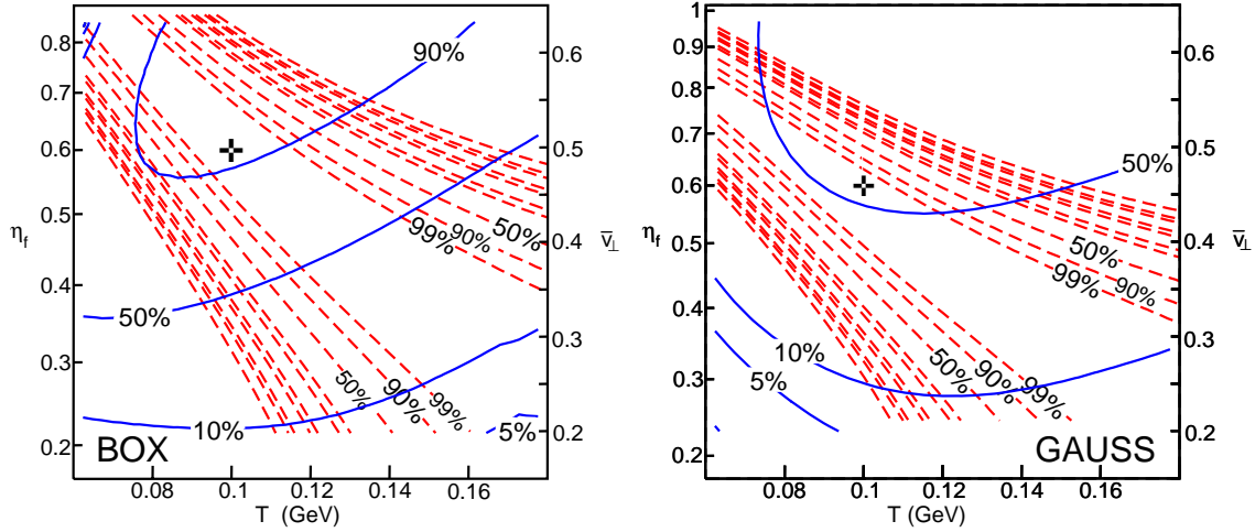
Figure 1. \chi^2 contours resulting from the fits to the single-particle m_{\perp} -spectrum of h^{-} [8] (dashed) and the two-particle correlations (solid). The contours correspond to the indicated confidence levels. The two plots are obtained with different transverse density profiles. Crosses show the positions of parameter sets used in comparative calculations.
