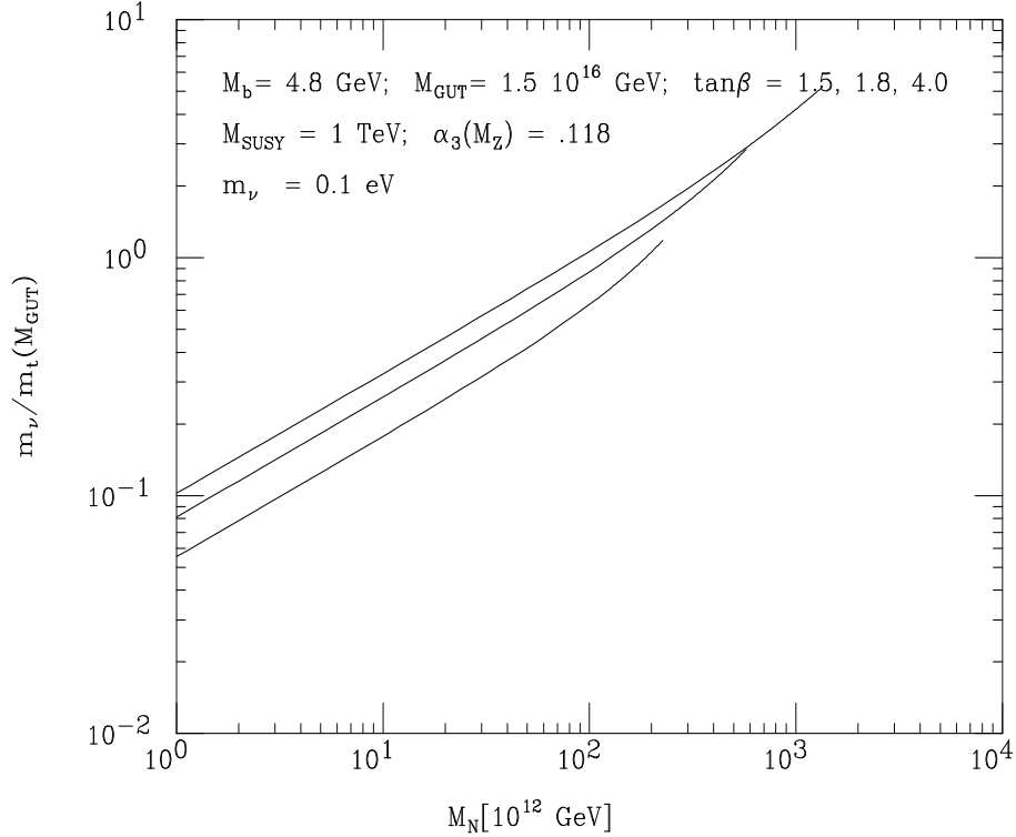
Figure 5: The ratio m_\nu/m_t(M_{GUT}) as a function of M_N , with the choice m_\nu = 0.1 \text{ eV} , for the same values of \tan\beta , from bottom to top, as in Fig. 1.
