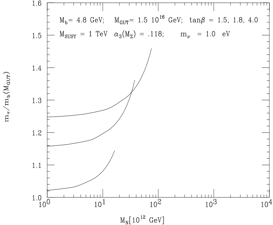
Figure 3: The ratio m_\tau/m_b(M_{GUT}) as a function of M_N , with the choice m_\nu = 1 eV, for the same values of \tan\beta , from bottom to top, as in Fig. 1.
