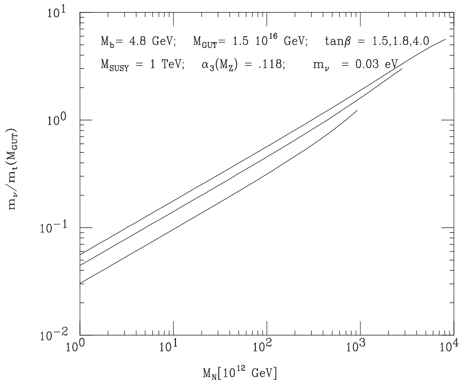
Figure 4: The ratio m_\nu/m_t(M_{GUT}) as a function of M_N , with the choice m_\nu = 0.03 eV, for the same values of \tan\beta , from bottom to top, as in Fig. 1.
