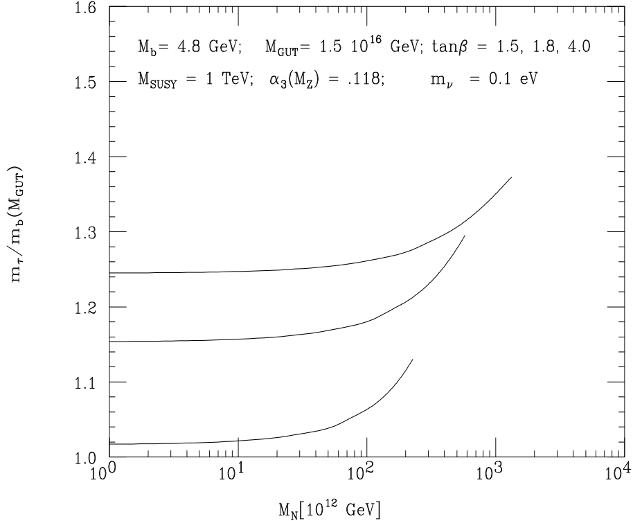
Figure 2: The ratio m_\tau/m_b(M_{GUT}) as a function of M_N , with the choice m_\nu = 0.1 eV, for the same values of \tan\beta , from bottom to top, as in Fig. 1.
