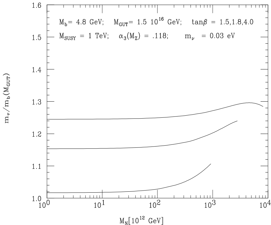
Figure 1: The ratio m_\tau/m_b(M_{GUT}) as a function of M_N , with the choice m_\nu = 0.03 eV and for different values of \tan\beta : from bottom to top, \tan\beta = 1.5, 1.8 and 4 , respectively.
