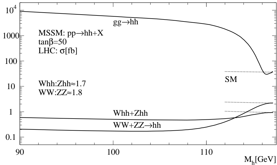
Figure 5b: Total cross sections for MSSM hh production via double Higgs-strahlung Whh , Zhh , WW/ZZ fusion and gluon fusion at the LHC for \tan\beta = 50 , including mixing effects ( A = 1 TeV, \mu = 1 TeV).
