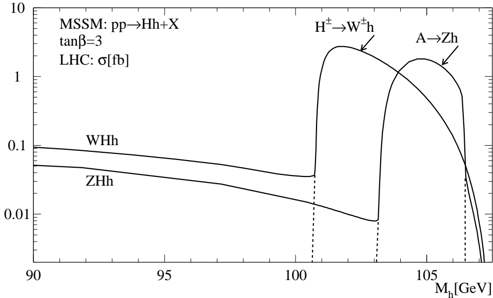
Figure 6: Total cross sections for MSSM Hh production in the processes WHh and ZHh for \tan\beta = 3 , including mixing effects ( A = 1 \text{ TeV} , \mu = -1 \text{ TeV} ).
