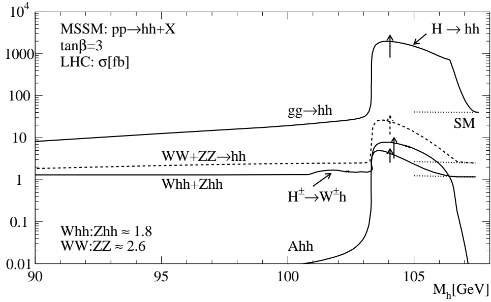
Figure 5a: Total cross sections for MSSM hh production via double Higgs-strahlung Whh and Zhh , WW/ZZ fusion and gluon fusion at the LHC for \tan\beta = 3 , including mixing effects ( A = 1 TeV, \mu = -1 TeV).
