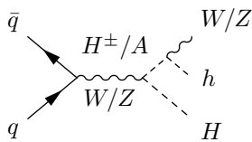
Figure 3: Processes which contribute to double light plus heavy Higgs production in the MSSM but which do not involve trilinear couplings.
