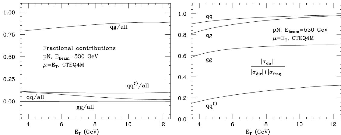
Figure 13: Left: relative contribution of different initial states to the E_T distribution in pN collisions at E_{\text{beam}} = 530 GeV. Right: relative size of the direct contribution vs. the sum of direct and fragmentation one, for the different channels.
