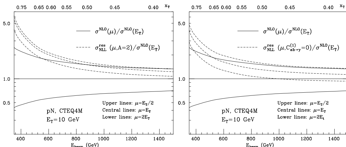
Figure 10: As fig. 9, but with with A = 2 (left panel) and with C_{ab\rightarrow\gamma}^{(1)} = 0 (right panel).
