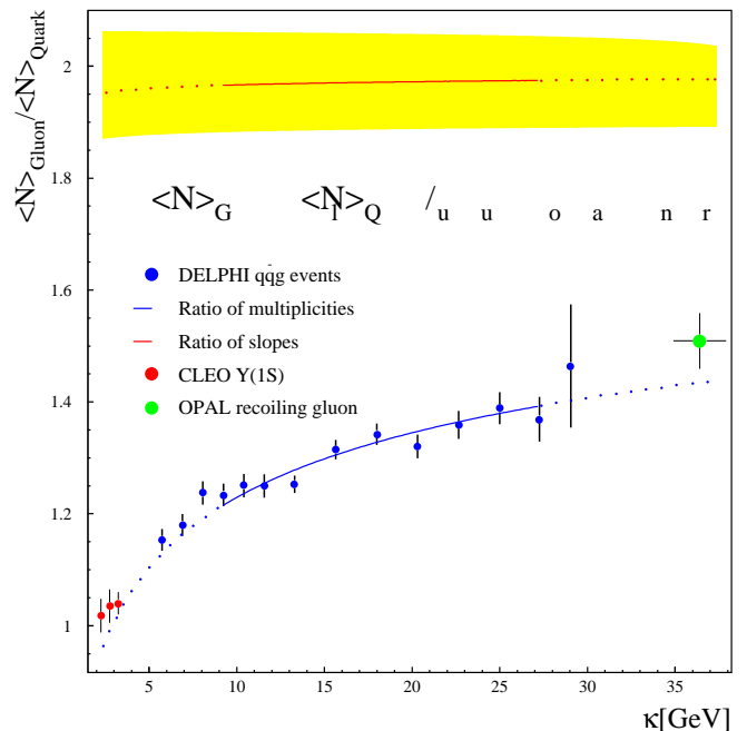
FIG. 9. Ratio of gluon and quark jet multiplicities and their slopes as a function of \kappa_H
