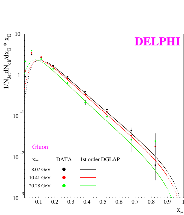
FIG. 4. Gluon fragmentation functions for different values of \kappa_H
