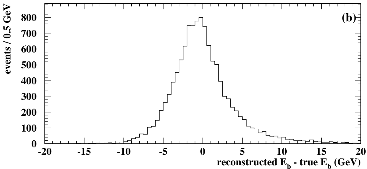
Figure 4: (a) Reconstructed b hadron energy distributions for data (points with error bars) and Monte Carlo (histogram). The position of the minimum energy cut is shown by the arrow. (b) Resolution of the reconstructed b hadron energy in Monte Carlo b\bar{b} events, after the minimum energy cut has been applied.
