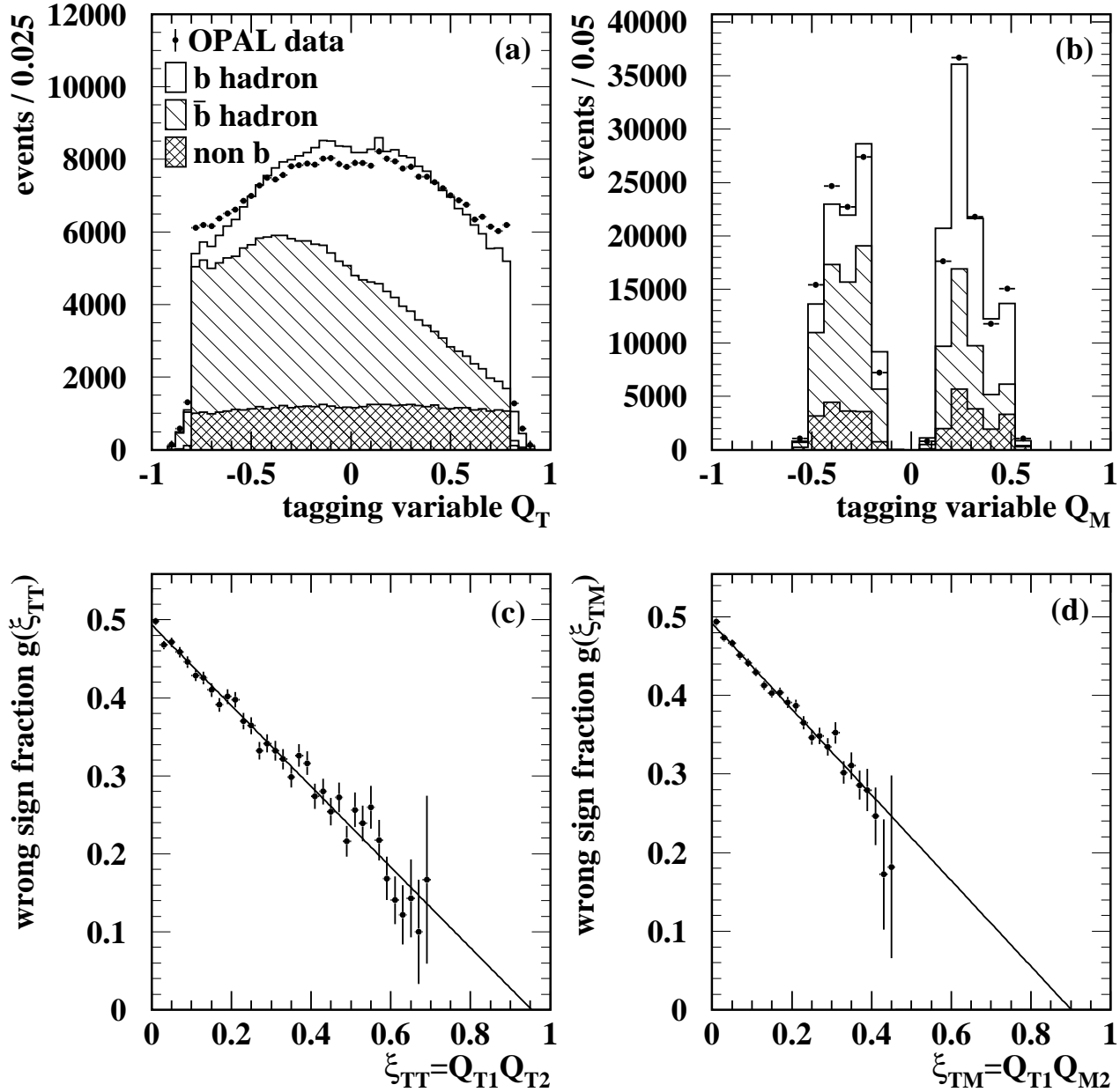
Figure 1: Production flavour tagging of b\bar{b} events: (a) Distribution of the flavour tagging variable Q_T in data (points) and Monte Carlo (histogram) T-tagged hemispheres. The contributions from b hadrons, \bar{b} hadrons and non-b backgrounds are shown. (b) The analogous distributions for the M-tag hemispheres. The 30% of the sample (90000 events in data) with Q_M = 0 are not shown. In both (a) and (b), the error bars on the data points are smaller than the symbols. (c) Distribution of the wrong sign fraction g(\xi_{TT}) in data double T-tagged events, with a linear fit superimposed. (d) Distribution of the wrong sign fraction g(\xi_{TM}) in data double T-tagged events, again with a linear fit superimposed.
