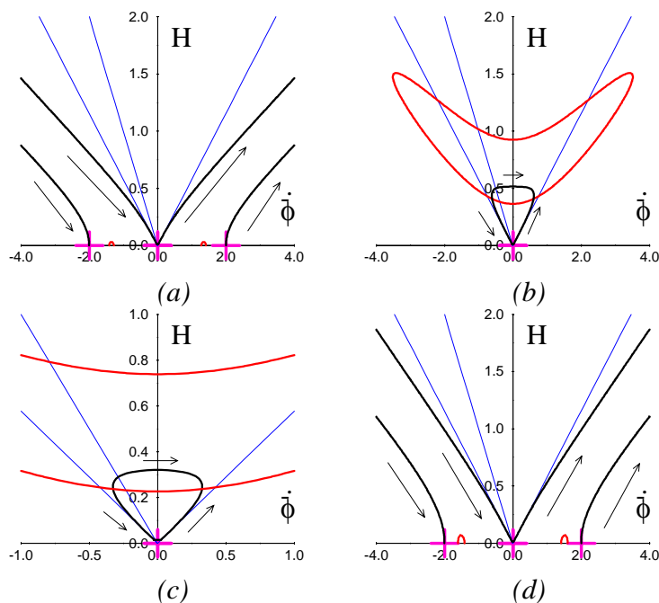
Figure 2: Sample evolutions of corrections constrained by (2.28). Features plotted are explained in fig. 1. (a) A=1/2 , B=1/2 . (b) A=-1/2 , B=1/2 . (c) A=-1/2 , B=-1/2 . (d) A=1/2 , B=-1/2 .
