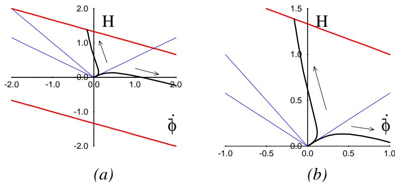
Figure 6: (a) Trajectories coming from the (+) vacuum, K=1 , for effective actions that contain (3.11) as a solution. The red lines are the lines of fixed points created by (3.11) (below) and its time reversed partner (above). (b) A closer view of (a) showing the solution going to a fixed point on the line created by the time reversed partner of (3.11).
