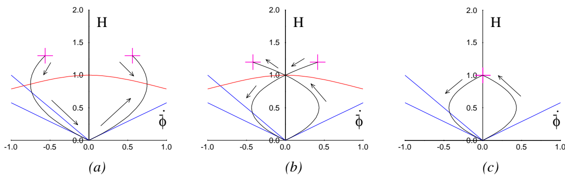
Figure 3: Possible cases of evolution to and from fixed points in the case of a self dual action.
