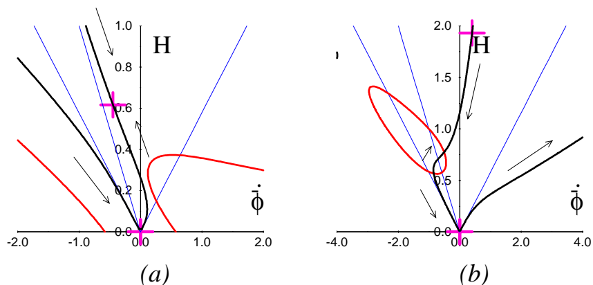
Figure 1: Sample evolutions in the (\dot{\phi}, H) phase space. The three blue lines are from left to right, the (-) branch vacuum, the Einstein frame bounce line and the (+) branch vacuum. The H axis is the line of branch change. The black line marked with arrows is the constraint curve (2.2) with the arrows indicating flow direction. Fixed points are marked with magenta crosses and the red curve indicates lines of singularities where the denominator of the expression for \dot{H} and \ddot{\phi} in terms of lower derivatives vanishes. (a) The effect of the O(\alpha') corrections in [10], A = -1/2, B = 1/2, C = 0, D = 0 . (b) The effect of the correction of [14] A = -1/2, B = 1/2, C = -2, D = 1 .
