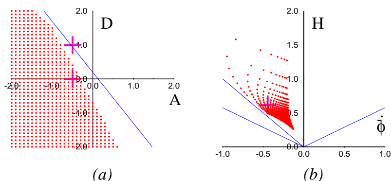
Figure 4: (a) The distribution of coefficients leading to good fixed point behavior in the (A, D) plane. C and D are chosen to fit the constraints (2.24) and (2.25). The line plotted is the condition of (2.27), to the right of this line solutions turn away from branch change and are not expected to lead to good fixed point behavior. The crosses marks the location of the corrections figured in fig. 1. (b) The location in the (\dot{\phi}, H) plane of the resulting good fixed points. The cross marks the location of the fixed point shown in fig. 1a.
