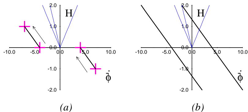
Figure 5: (a) The CFT trajectory, K=1 , on the left and its time reversed partner on the right, with beginning and ending fixed points marked. (b) The CFT trajectory extended to include all of the fixed points allowed by the equations of motion from an effective action.
