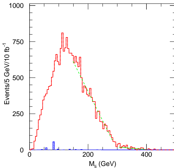
Figure 20: M_{l_j} mass spectrum at Point G2a. The fits shown as dashed lines correspond to two separate linear fits over the ranges is over the ranges 150 to 280 GeV and 305 to 400 GeV. The former extrapolates to an endpoint at 315 GeV. The Standard Model background is shown as the hatched histogram.
