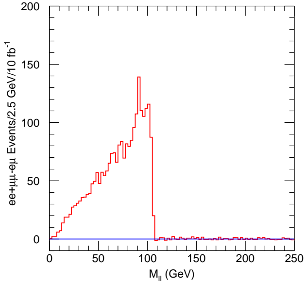
Figure 1: M_{\ell\ell} distribution for e^+e^- + \mu^+\mu^- - e^\pm\mu^\mp events with two photons and two isolated leptons arising at Point G1a. The Standard Model background is negligible.
