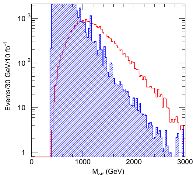
Figure 10: The effective mass distribution showing LHC Point G1b signal and Standard Model backgrounds (hatched histogram)
