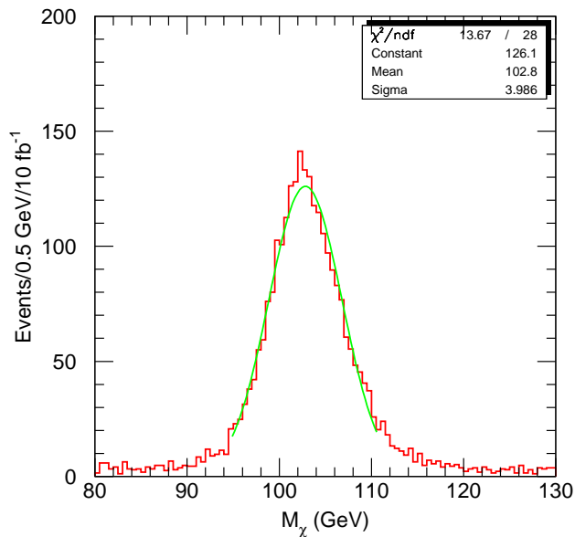
Figure 28: Same as Figure 26 for events in a \pm 5 GeV window around the \tilde{\chi}_1^0 mass peak of Figure 27 and the lepton is identified as an electron.
