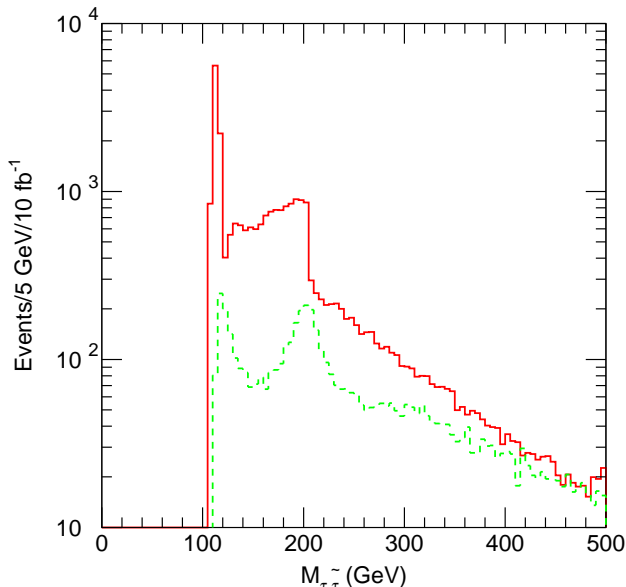
Figure 32: \tilde{\tau} - \tau mass distribution at Point G2b. Solid curve: Using visible \tau momentum. The dotted curve is obtained by selecting events where the missing E_T is aligned with the tau direction by \Delta\phi < 0.1\pi and adding \cancel{E}_T to \tau momentum.
