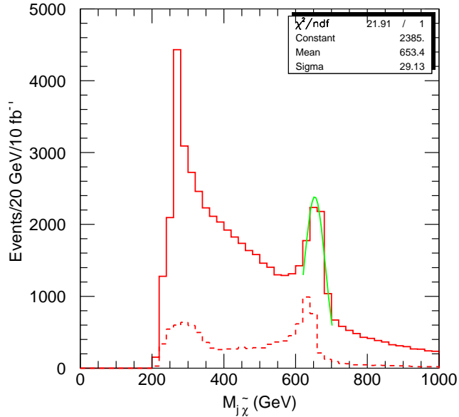
Figure 31: \tilde{\chi}_2^0 - q mass distribution at point G2b. Events have a lepton and a slepton with invariant mass in a \pm 5 GeV window around the \tilde{\chi}_2^0 . The dashed distribution corresponds to cases where the jet is from a b -quark. The fit is a Gaussian over the range 625 to 700 GeV
