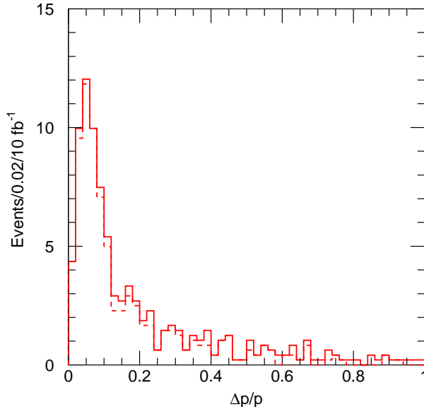
Figure 4: The distribution in |\Delta p|/|p| for reconstructed gravitino momenta. The gravitino momenta are reconstructed using the method described in the text. The difference ( \Delta p ) between the reconstructed ( p ) and generated momentum is then formed for the combination with the lowest \chi^2 . Events are included where the lowest \chi^2 is less than 10 or 1 (dashed line).
