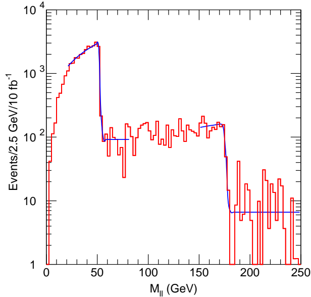
Figure 18: As Figure 16 except that the distribution is shown on a logarithmic scale and the fits to the edges described in the text are shown. No background is shown on this figure.
