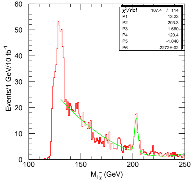
Figure 35: The mass of the slepton-lepton-lepton system formed by selecting events in the mass range 110–120 GeV from Figure 34 and combining this slepton-lepton pair with and additional lepton.
