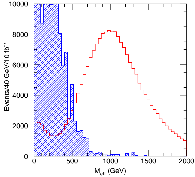
Figure 24: Effective mass distribution not including sleptons at Point G2b. The Standard Model background of dimuon events is shown as the hatched histogram.
