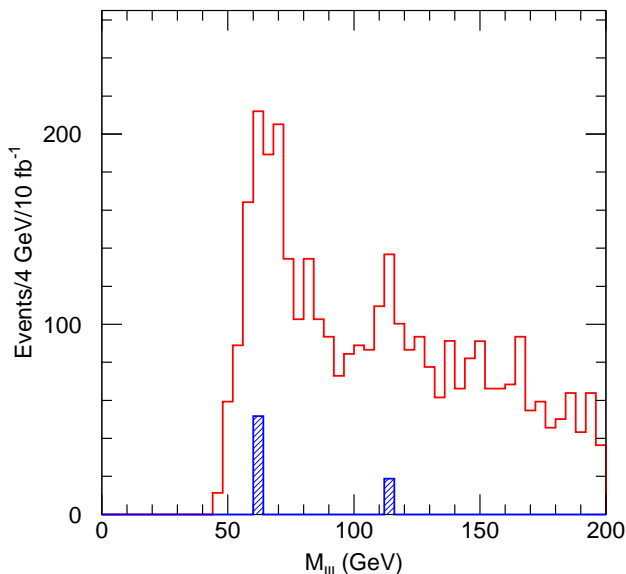
Figure 21: M_{\ell\ell\ell} mass spectrum at Point G2a. The Standard Model background (hatched histogram) is very small.
