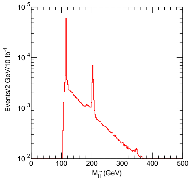
Figure 27: \tilde{\ell}^{\pm}\ell^{\mp} mass distribution at Point G2b.
