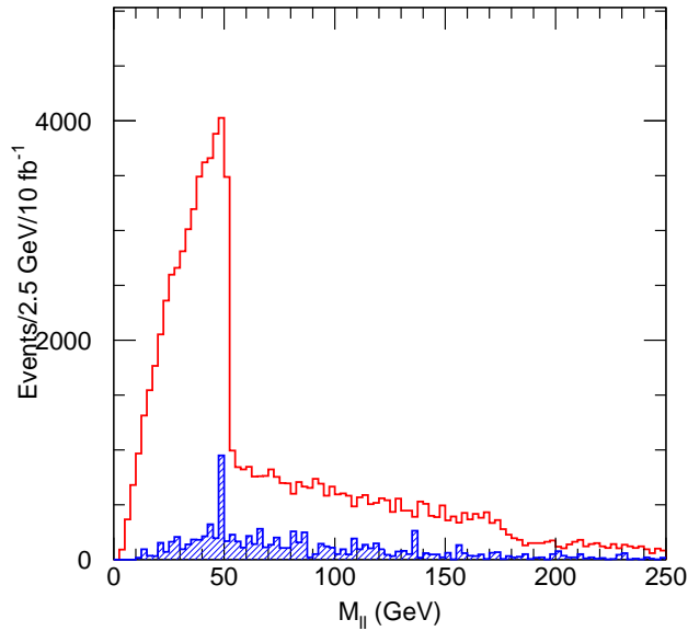
Figure 17: M_{\ell\ell} distribution for all oppositely charged dilepton pairs e^+e^- + \mu^+\mu^- + e^\pm\mu^\mp in events having two isolated leptons arising at Point G2a. The background, mostly from t\bar{t} production, is shown as the hatched histogram.
