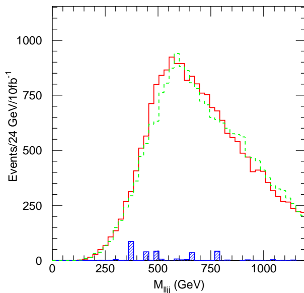
Figure 12: The mass distribution of a dilepton and two jets at Point G1b. The dotted histogram corresponds to a different event sample where the gluino mass is changed to 800 GeV, this distribution has been scaled by a factor of 1.24 to facilitate comparison of the shapes. The Standard Model background is shown as the hatched histogram.
