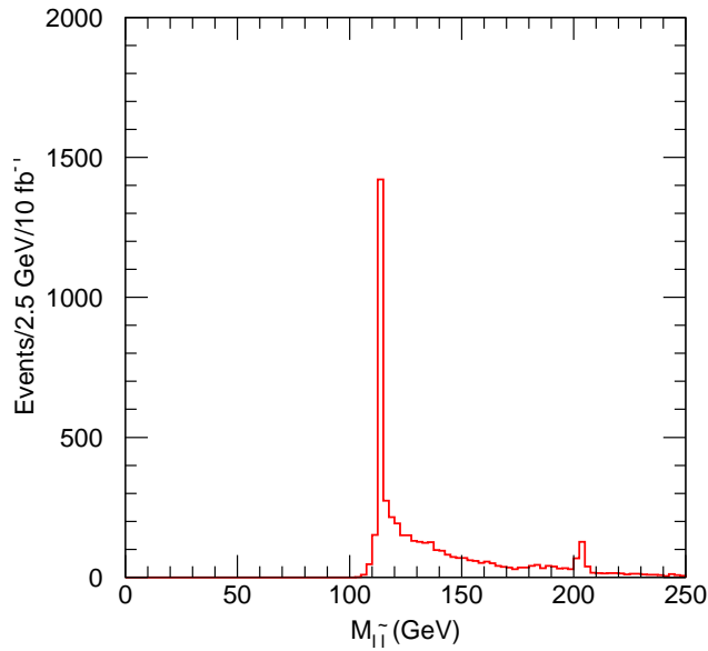
Figure 34: Same as Figure 28 except that the additional requirement M_{\text{eff}} < 100 GeV has been made.
