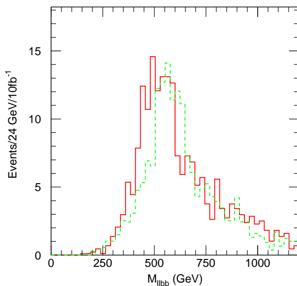
Figure 13: The mass distribution of a dilepton and two b-jets at Point G1b. The dashed histogram corresponds to a different event sample where the gluino mass is changed to 800 GeV. No standard model background events passed the cuts.
