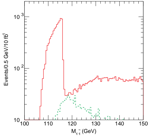
Figure 33: Same as Figure 32 on a finer scale with smaller bins.
