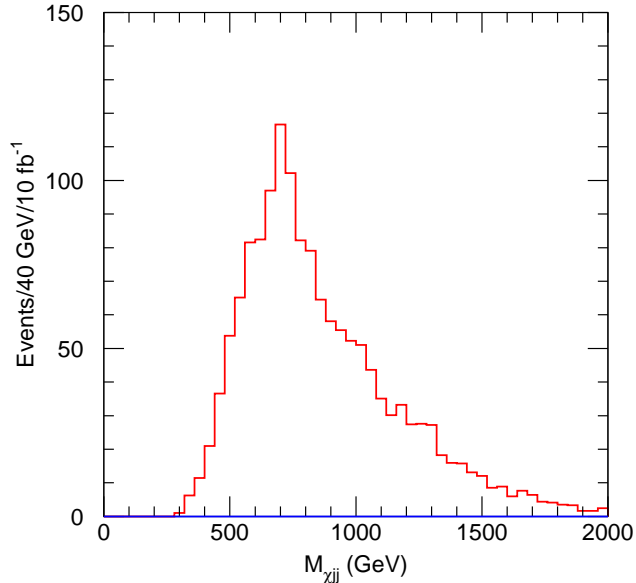
Figure 5: Invariant mass of \tilde{\chi}_2^0 and two jets, for events at Point G1a. The peak is due to the decay \tilde{g} \rightarrow q\bar{q}\tilde{\chi}_2^0 . Events are required to have two \tilde{\chi}_2^0 momenta reconstructed and at least four jets with p_T > 75 GeV.
