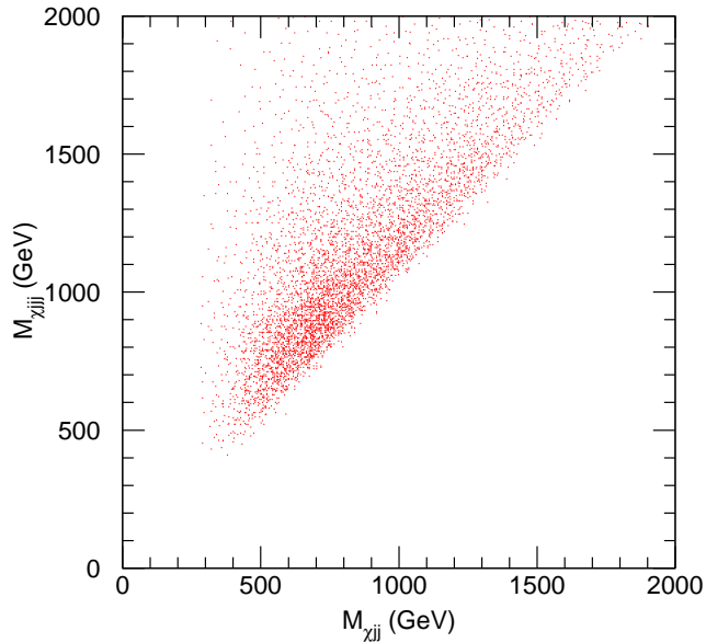
Figure 7: Scatter plot of M(\tilde{\chi}_2^0 jjj) vs. M(\tilde{\chi}_2^0 jj) for events at Point G1a where two \tilde{\chi}_2^0 momenta are reconstructed and there are at least four jets with p_T > 75 GeV.
