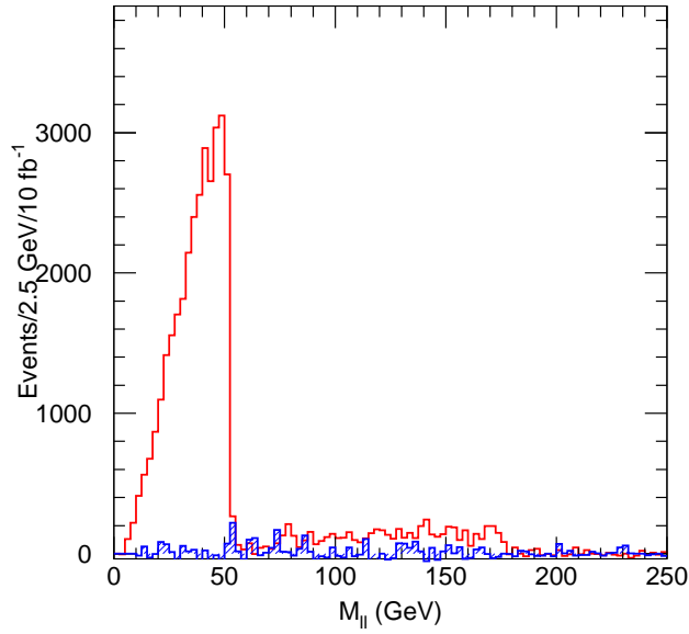
Figure 16: M_{\ell\ell} distribution for the flavor subtracted combination e^+e^- + \mu^+\mu^- - e^\pm\mu^\mp of events having two isolated leptons arising at Point G2a. The Standard Model background shown does not represent the statistical fluctuations expected in 10\text{ fb}^{-1} of integrated luminosity (see text).
