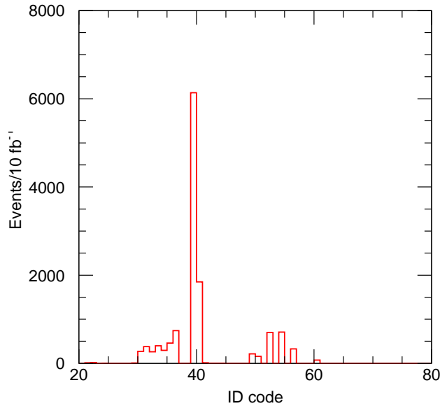
Figure 25: The particle ID codes for the primary particles of events in Figure 24 which have M_{\text{eff}} < 100 GeV: left sleptons (31-36), gauginos (30, 39 and 40) and right sleptons (52, 54, and 56).
