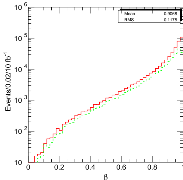
Figure 22: Generated slepton velocity distribution \beta at Point G2b. The dotted curve is for sleptons with \eta < 1 .
