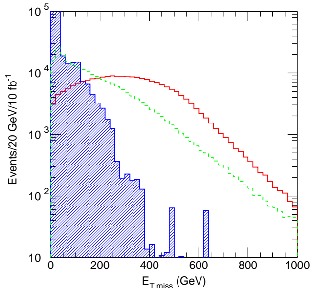
Figure 23: Calorimetric missing transverse energy \cancel{E}_T at Point G2b. The dotted curve shows the true \cancel{E}_T including sleptons. The Standard Model background of dimuon events is shown as the hatched histogram.
