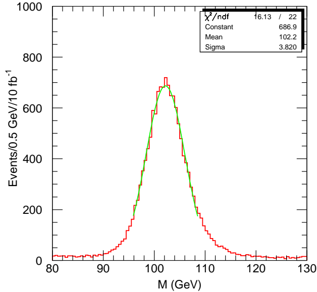
Figure 26: Reconstructed slepton masses for time delays 10 \text{ ns} < \Delta t < 50 \text{ ns} relative to a \beta = 1 particle.
