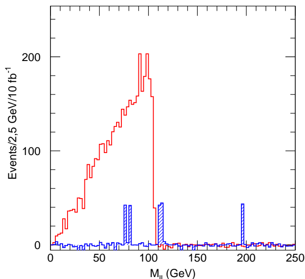
Figure 11: The dilepton mass distribution at Point G1b. The Standard Model background (hatched histogram) is very small. The fluctuations in our event sample for the combination shown i.e. e^+e^- + \mu^+\mu^- - e^\pm\mu^\mp are therefore larger than one would expect in 10 \text{ fb}^{-1} .
