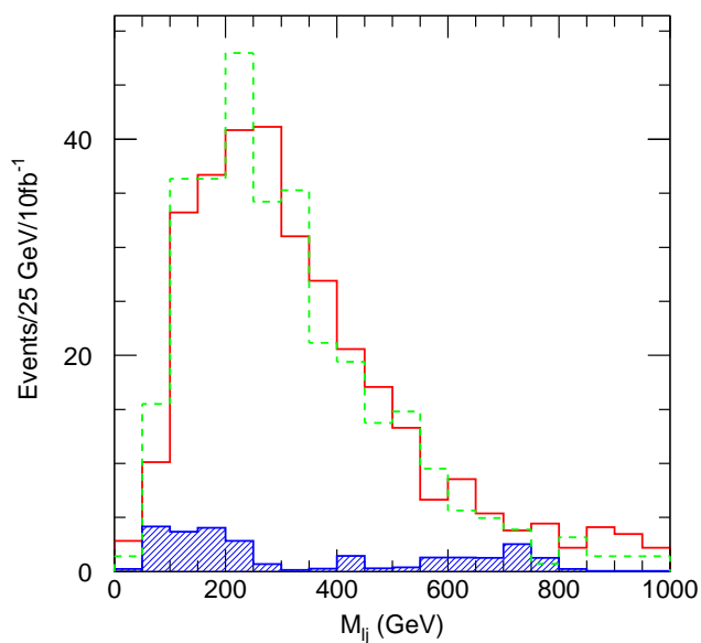
Figure 15: The mass distribution of a lepton+jet system. The dashed histogram corresponds to a different event sample where the squark mass has been reduced by 50 GeV. The Standard Model background shown as a hatched histogram is dominated by t\bar{t} production.
