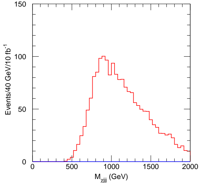
Figure 6: Invariant mass of \tilde{\chi}_2^0 and three jets, for events at Point G1a. The peak is due to the decay \tilde{q} \rightarrow q\tilde{g} \rightarrow qq\bar{q}\tilde{\chi}_2^0 .
