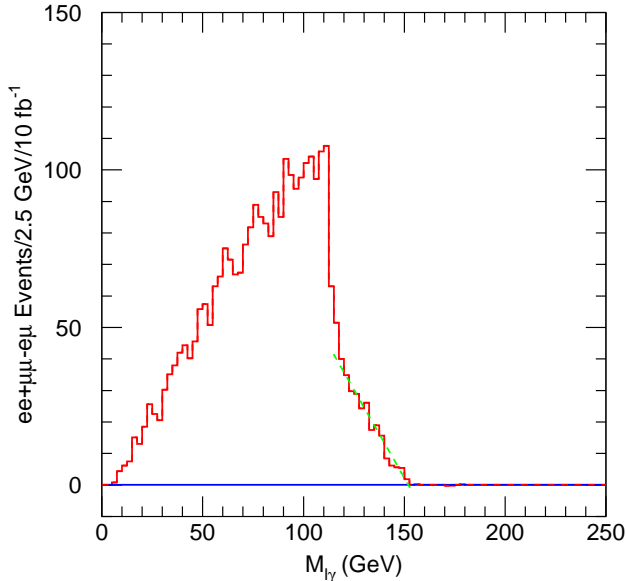
Figure 3: M_{\ell^\pm\gamma} distribution for e^+e^- + \mu^+\mu^- - e^\pm\mu^\mp events sample with two photons; a linear fit from 115 to 150 GeV is used to determine the endpoint for the photon and the “wrong” lepton and is shown as a dashed line.
