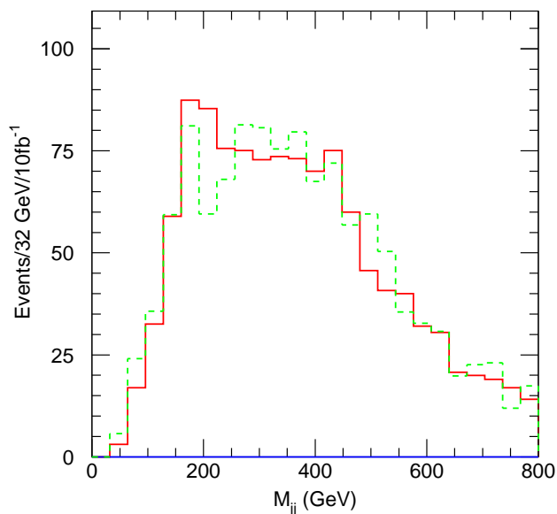
Figure 14: The mass distribution of two jets at Point G1b. There are two entries per event. The dotted histogram corresponds to a different event sample where the gluino mass is changed to 800 GeV, this distribution has been scaled by a factor of 1.18 to facilitate comparison of the shapes. No Standard Model events passed the cuts.
