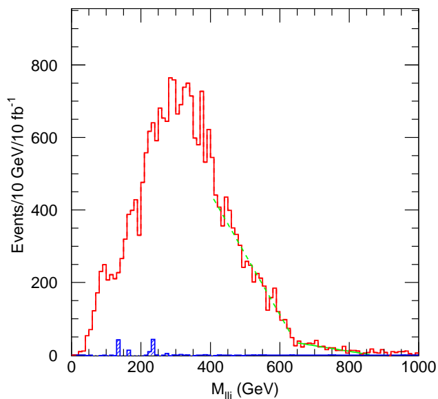
Figure 19: M_{\ell\ell j} mass spectrum at Point G2a for events that contain at least two isolated leptons and four jets. The linear fit shown as a dashed line is over the range 390 to 590 GeV. The Standard Model background is shown as the hatched histogram.
