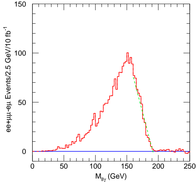
Figure 2: M_{\ell\ell\gamma} distribution for e^+e^- + \mu^+\mu^- - e^\pm\mu^\mp events with two photons at Point G1a. A linear fit from 160 to 190 GeV used to determine the position of the 4-body endpoint is also shown as a dashed line.
