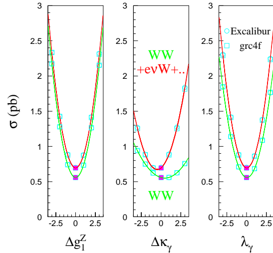
Figure 4: Sensitivity of the cross sections to \Delta g_1^Z , \Delta\kappa_\gamma and \lambda_\gamma with and without inclusion of the single W processes.
