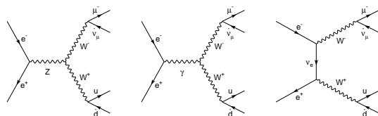
Figure 1: Signal diagrams for e^+e^- \rightarrow \mu\nu_\mu u\bar{d} .
