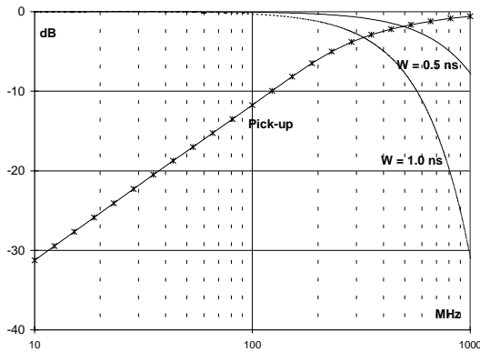
FIGURE 4A. Frequency spectrum & PU response
