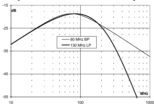
FIGURE 5. Filters frequency response
