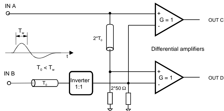
FIGURE 7. Inverter Normalizer
