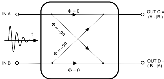
FIGURE 1. Phase Normalizer schematics
