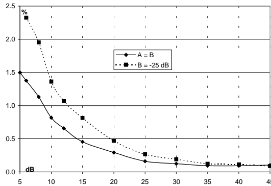
FIGURE 11. Normalized Noise vs. input level above threshold
