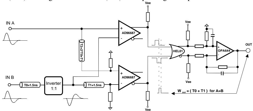
FIGURE 8. Wide Band Normalizer block diagram
