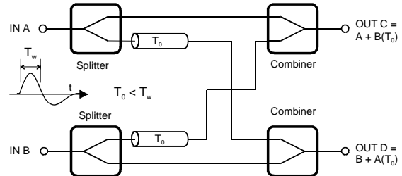
FIGURE 2. Time Normalizer schematics
