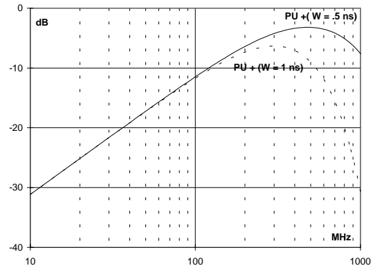
FIGURE 4B. Pick-up output spectrum content
