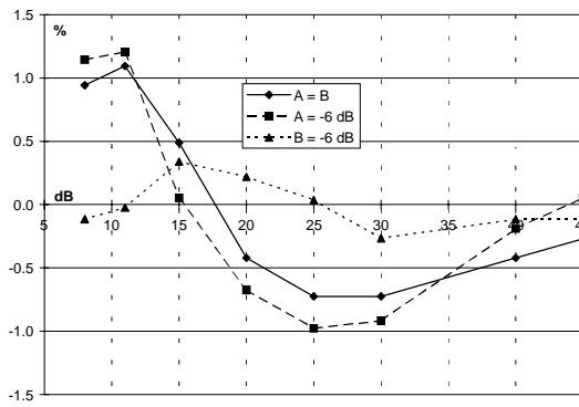
FIGURE 9. Normalized out variation vs. overdrive
