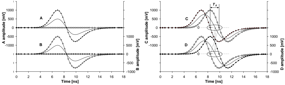
FIGURE 3. Signals at Normalizer inputs (left) and outputs (right) for three different beam positions
