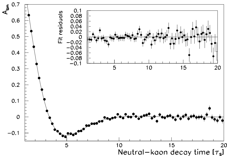
Figure 2: The asymmetry A_{\Delta m} versus the neutral-kaon decay time (in unit of \tau_S ). The solid line represents the result of the fit.
