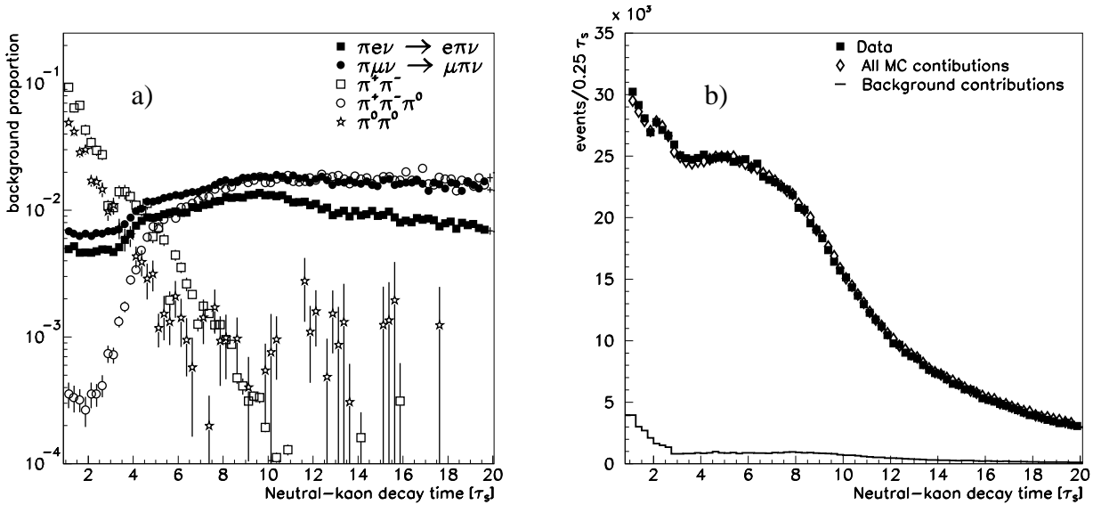
Figure 1: a) Proportion of different background channels relative to the semileptonic signal. b) Decay-time distribution for real data (squares) and simulated data (open diamonds). The expected background contribution is shown by the solid line.
