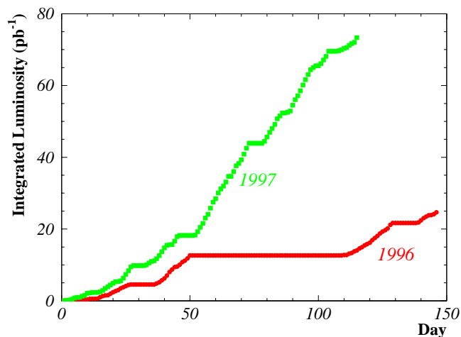
Figure 1: Evolution of the integrated luminosities during the 1996 and 1997 LEP runs. When the best periods of the two runs are compared, the slope for 1997 is a factor 2.3 steeper than for 1996.
