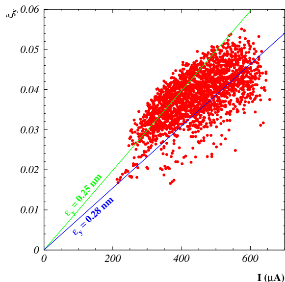
Figure 3: Vertical beam-beam tune shift \xi_y as a function of the bunch current ( \beta_x^* = 1.5 \text{ m} ). There is no strong evidence for a beam-beam limit. The lines show the expected dependences for two vertical emittances \varepsilon_y .
