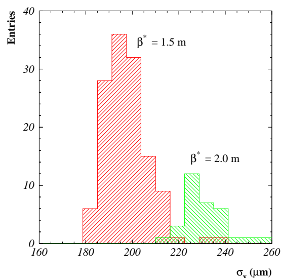
Figure 2: Horizontal beam sizes \sigma_x measured with beam-beam deflections scans for \beta_x^* = 1.5 and 2.0 \text{ m} ( J_x = 1.6 ). The mean ratio is 1.15 as expected from the \beta_x^* ratio.
