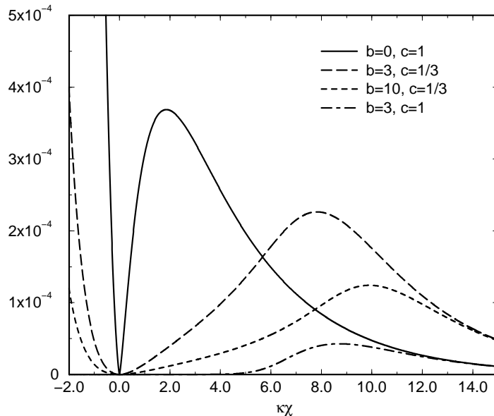
Figure 2: The potential from Eq. (41) for different values of the parameters b and c controlling the relative strengths of the R^2 and R^4 terms in the five-dimensional action.
