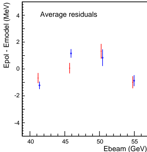
Figure 6: Residual beam energy variations for different beam energies comparing the resonant depolarization calibrations and the beam energy estimated using NMR probes.
