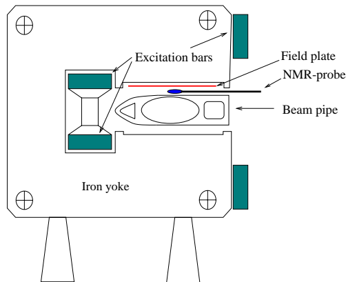
Figure 1: Cross section of the instrumented LEP dipole. The NMR probe is mounted in top of the chamber and below the field plate, which is glued on the pole surface.
