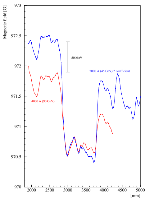
Figure 5: Variation of the field of the LEP iron concrete core magnet along the gap.
