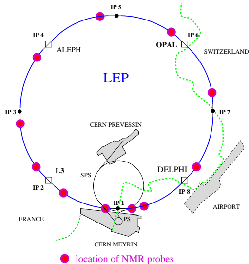
Figure 2: Location of the NMR probes around LEP. The probes left and right of point 1 are installed in the LEP injection magnets (iron core with twice the field of standard magnets). The location near point 3 is equipped with four probes for special test measurements.
