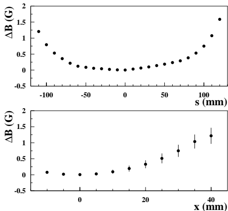
Figure 3: Variation of the magnetic field just below the field plate in the gap of the bending magnet as function of the longitudinal ( s ) and transverse ( x ) extension of the magnet.
