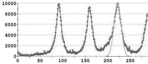
Fig. 7: Vertical projection of acquired beam images, together with the gaussian fit of the third profile. The units on the x-axis are in pixels [500 \mu\text{m}/\text{px} ].
