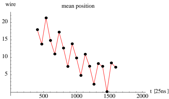
Fig. 4: Position oscillations. Each point corresponds to one beam passage through the SEM grid.
