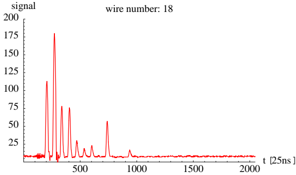
Fig. 2: Signal on a single wire. Each peak corresponds to one turn in the accelerator.
