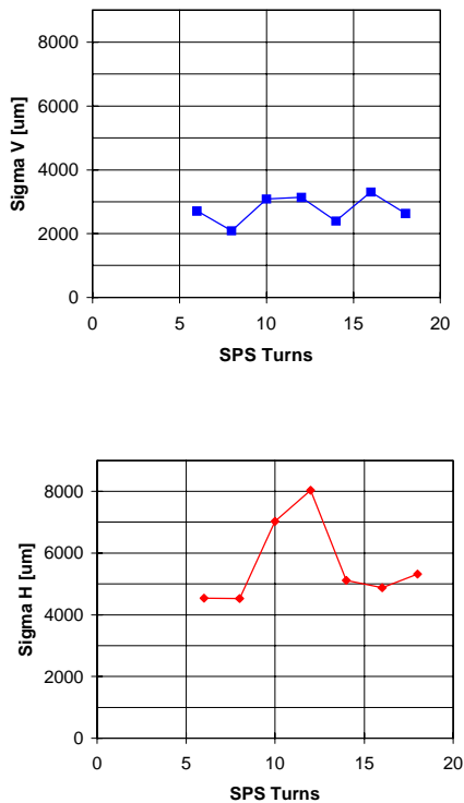
Fig.8: Horizontal and vertical beam size variation measured over 12 turns in the SPS: the matching is acceptable in the vertical direction and worse in the horizontal one.
