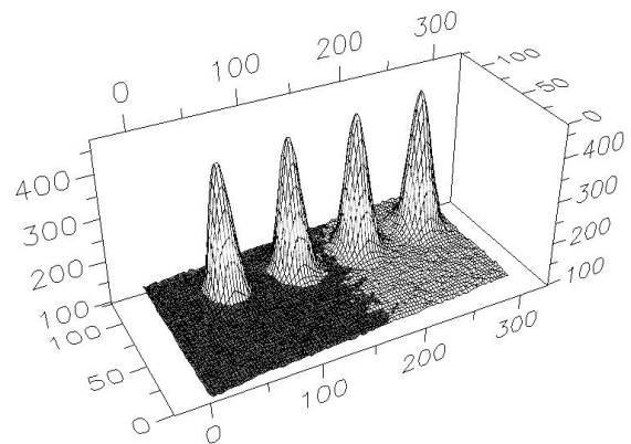
Fig. 6: Result of the digitisation of four beam images from successive SPS turns memorised on the CCD.
