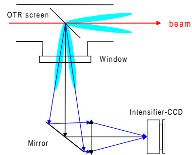
Fig.5: Matching monitor set-up in the SPS
