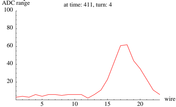
Fig. 3: The beam profile for one passage through the SEM grid.
