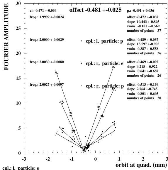
Figure 4: Example of a BPM calibration. The oscillation amplitude \Delta y is plotted as a function of the beam position in the quadrupole y_Q . The offset is given by the minimum oscillation amplitude. The different marker types indicate the four measurements for electrons and positrons in both detectors. The data of each measurement is fitted according to Eq. 5. The number of data points, results and uncertainties for each fit are also listed in the plot. The average offset is -481 \pm 25 \mu\text{m} .
