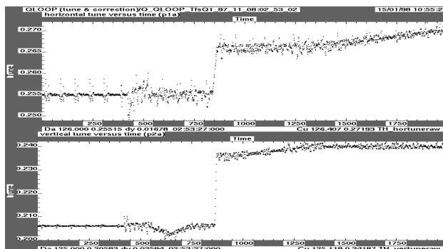
Figure 4: Horizontal and vertical tunes during the ramp
