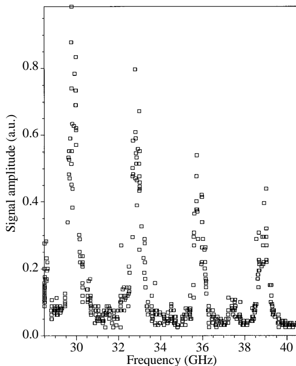
Figure 4: Measured frequency spectrum for a train of 8 bunches.
