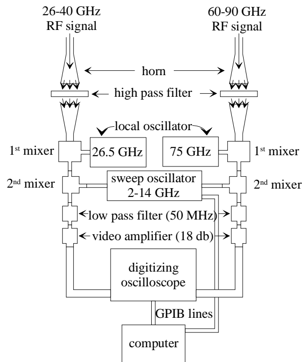
Figure 3: Detection system.
