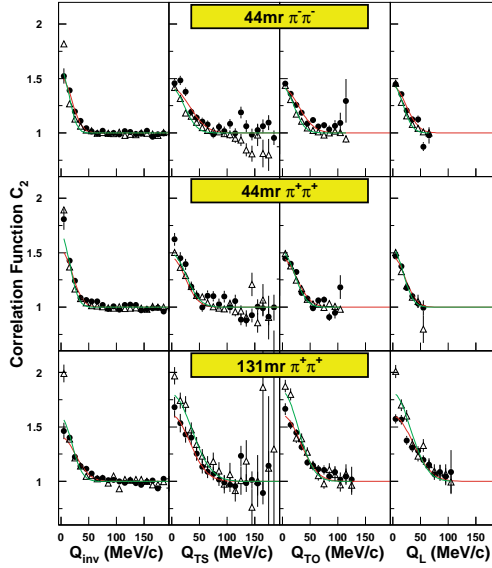
Figure 7: Comparison of NA44 data and RQMD predictions. The solid circles are the NA44 data and the open triangles are the RQMD predictions. The three-dimensional projections are averaged over the lowest 20 MeV/c in the other momentum differences.
