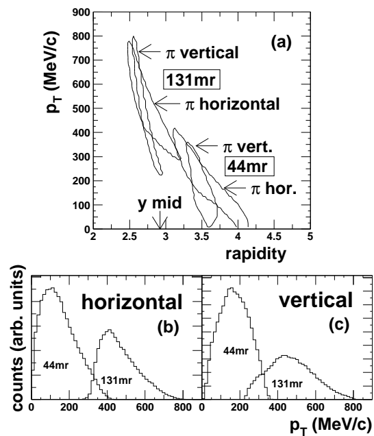
Figure 2: The NA44 pion acceptance for the 4 GeV/c 44 mrad and 131 mrad horizontal and vertical settings.
