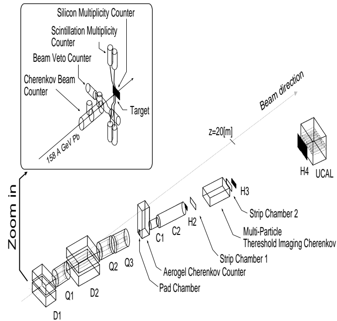
Figure 1: The NA44 spectrometer in 1995 and 1996.
