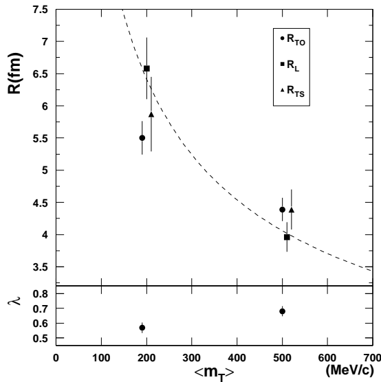
Figure 5: The m_T dependence of \pi^+\pi^+ radius and \lambda parameters. Also included is the fit of the R_L radius parameters to the function A/\sqrt{m_T} .
