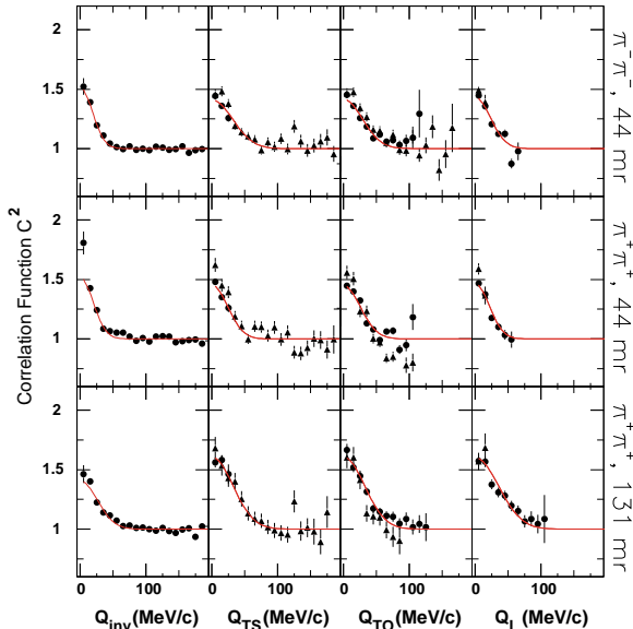
Figure 3: The one-dimensional correlation functions and the projections of the three-dimensional correlation functions for the 44 mrad \pi^-\pi^- , 44 mrad \pi^+\pi^+ and the 131 mrad \pi^+\pi^+ data. Also included are the projections of the fitted Gaussian parametrizations. The projections are over the lowest 20 MeV/ c in the other momentum-difference directions. The solid circles are the data from the horizontal setting and the solid triangles are the data from the vertical setting. The data shown here use the Coulomb wave-function integration correction.
