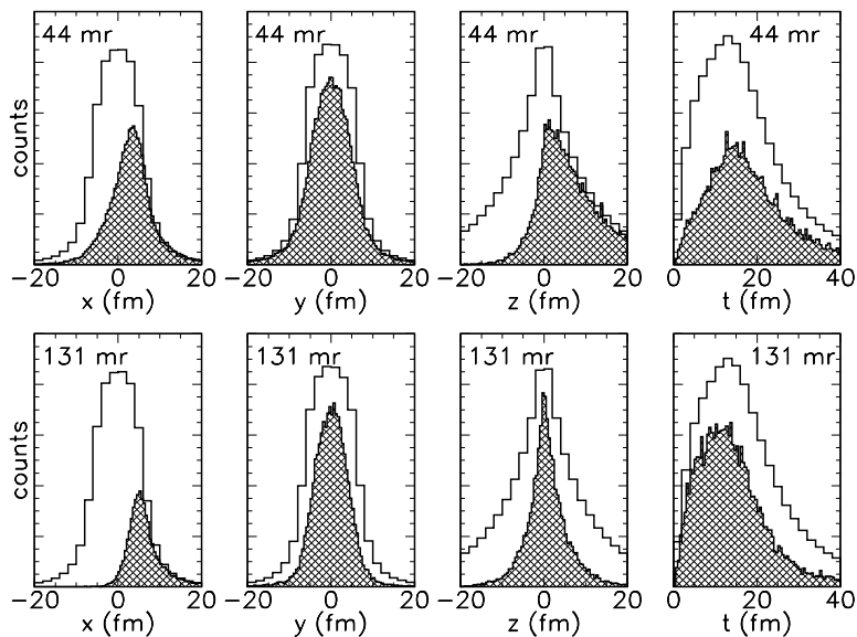
Figure 8: RQMD freeze-out distributions for pions. The unhatched histograms are for all pions from RQMD, and the hatched histograms are for pions in the NA44 44-mrad horizontal (upper panels) and 131-mrad horizontal (lower panels) acceptances. The x axis is in the direction of Q_{TO} , the y axis is in the Q_{TS} direction, and z is the beam axis. The centre-of-mass coordinate system is used.
