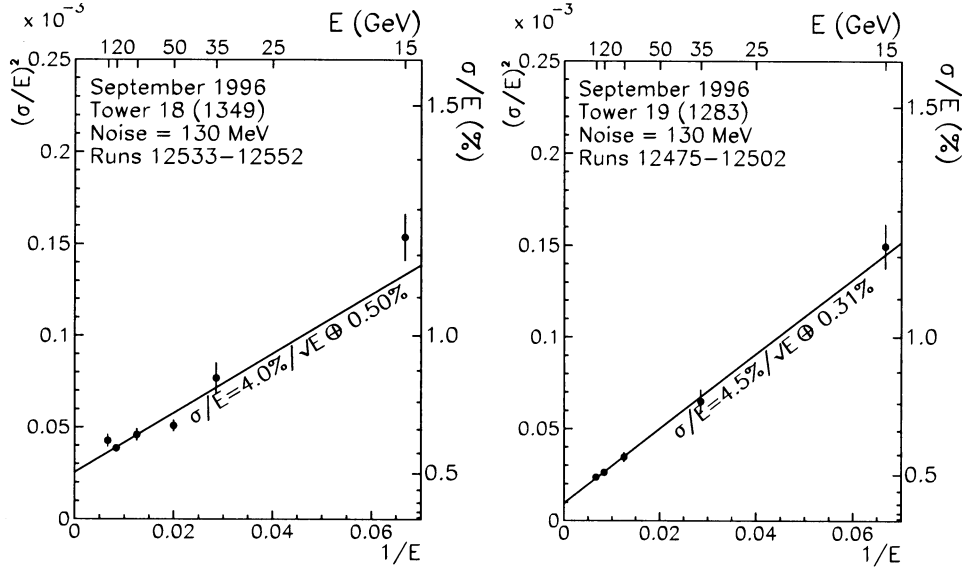
Figure 4: Fits to the energy resolution (noise subtracted) as a function of energy for beam incident in two adjacent crystals in the September matrix.
