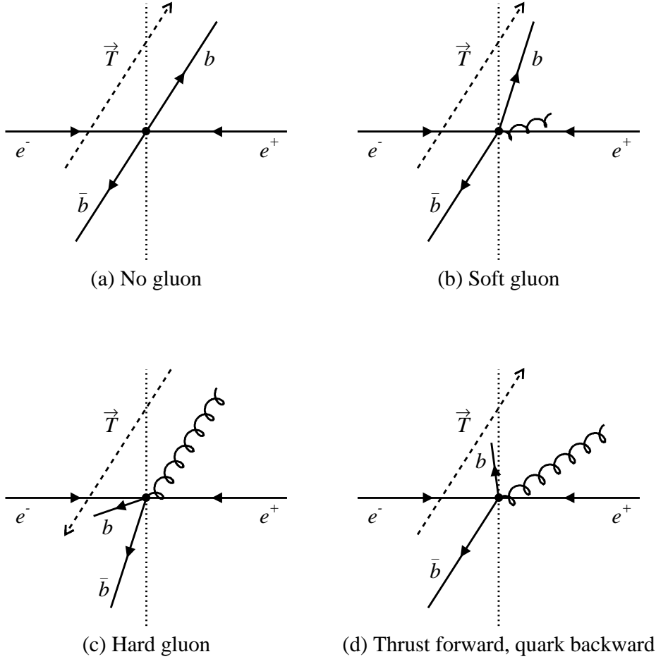
Figure 1: Pictorial representation of final state topologies with gluon emission. In this figure the thrust axis is oriented that \vec{T} \cdot \vec{p} > 0 , with \vec{p} corresponding to the quark direction. (a) The pure electroweak process. (b) “Soft” gluon radiation slightly changes the direction of the quark. The thrust axis is a good estimator of the primary b direction. (c) “Hard” gluon radiation flips the quark in the hemisphere of the anti-quark. No charge information is contained in the hemisphere of the gluon. (d) Another topology caused by hard gluon radiation is represented. The event is classified as “forward” when using the thrust direction even if the quark has flipped into the backward hemisphere.
