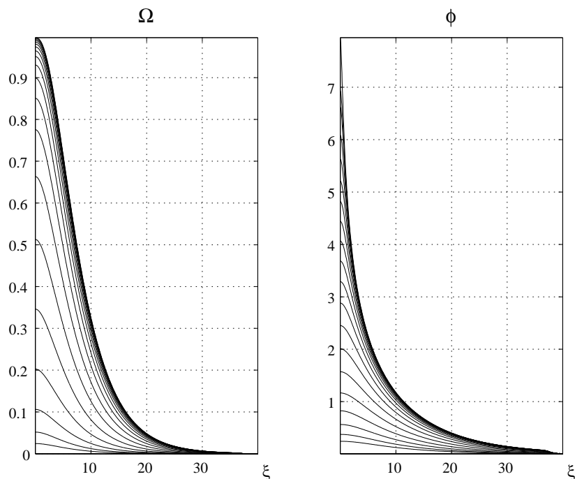
Figure 2: The \Omega parameter and the dilaton, same initial data as above.
