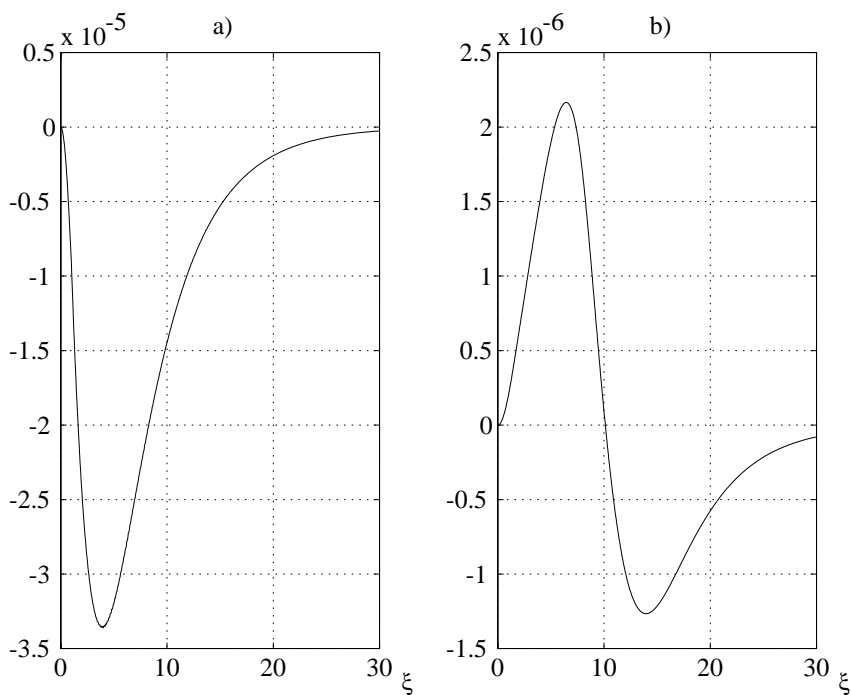
Figure 7: The function \lambda(\xi) , (a) \xi_0 = 0 , b) \xi_0 = 10 ).
