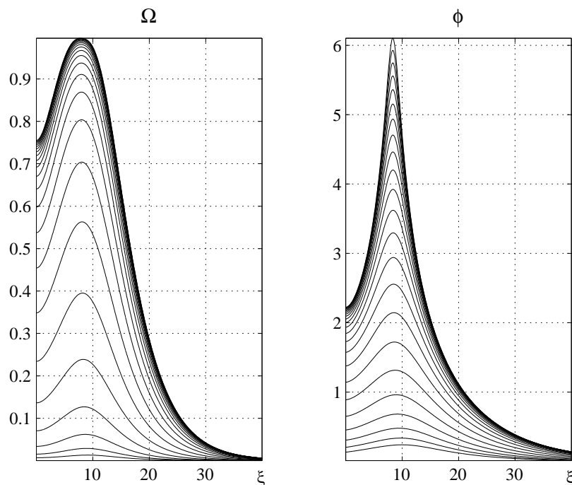
Figure 4: The \Omega parameter and the dilaton, same initial data as above.
