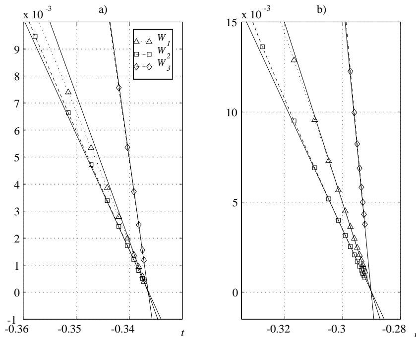
Figure 5: The asymptotic behaviour \mathcal{O}(t_0(\xi) - t) for the variables W_n at the \Omega peak ( a ) \xi_0 = 0 , b ) \xi_0 = 10 )
