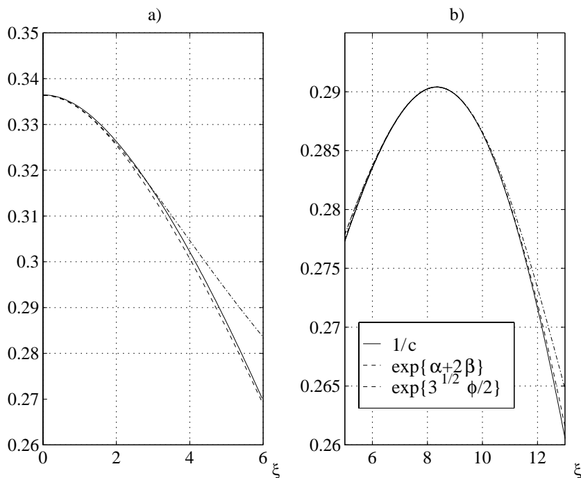
Figure 6: The blowing-up time t_0(\xi) , (a) \xi_0 = 0 , b) \xi_0 = 10 ).
