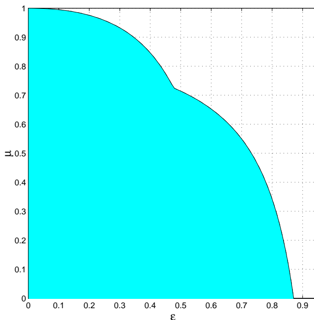
Figure 8: Admissible values for \mu, \varepsilon .
