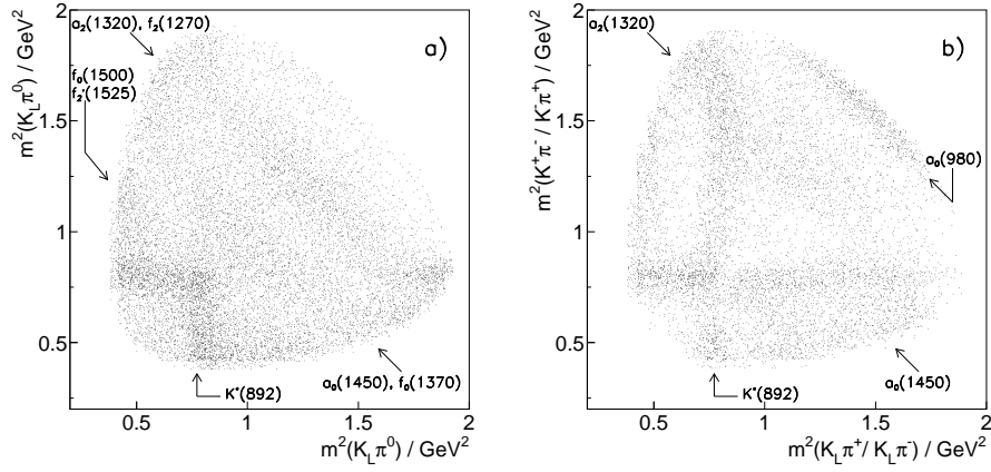
Fig. 1. The Dalitz plots for the annihilation reactions a) \bar{p}p \rightarrow K_L K_L \pi^0 and b) \bar{p}p \rightarrow K_L K^\pm \pi^m p in liquid hydrogen.
