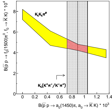
Fig. 2. Determination of the branching ratio of f_0(1500) in the reaction \bar{p}p \rightarrow K_L K_L \pi^0 [4] (light hatched area), where it is correlated with the a_0(1450) production. The a_0(1450) contribution is fixed in the analysis of the reaction \bar{p}p \rightarrow K_L K^\pm \pi^m p [6].
