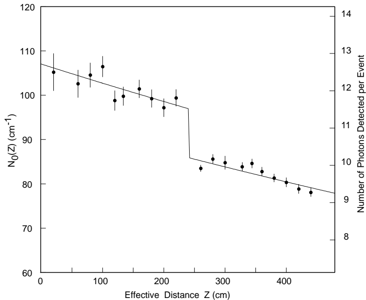
Figure 6: N_0 as a function of the effective bar transmission distance Z for the coarse Z scan at \theta_D = \pm 20^\circ and 5.4 \text{ GeV}/c momentum. Pion and proton samples are averaged in the data points shown. The discontinuity at Z = 240 \text{ cm} accounts for the end mirror reflectivity. A possible loss at the glue joint (for Z = 120 \text{ cm} and Z = 360 \text{ cm} ) was not included in this fit. The scale at the right indicates the average number of signal photons extracted from a ring fit in the range |\phi_C| < 1.0 \text{ rad} .
