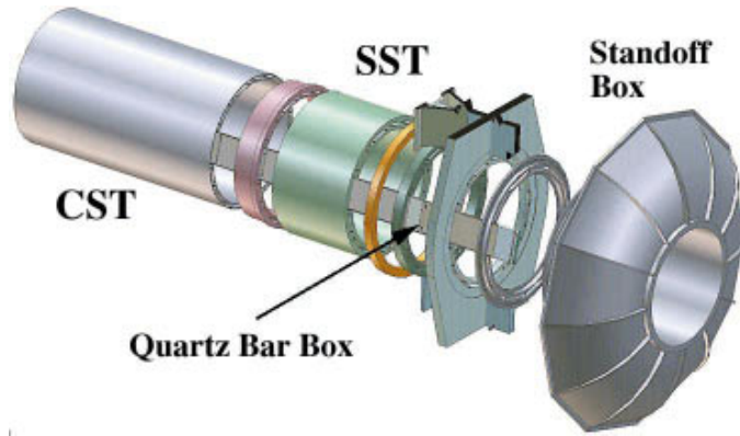
Figure 8: Schematic of the DIRC detector assembly.
