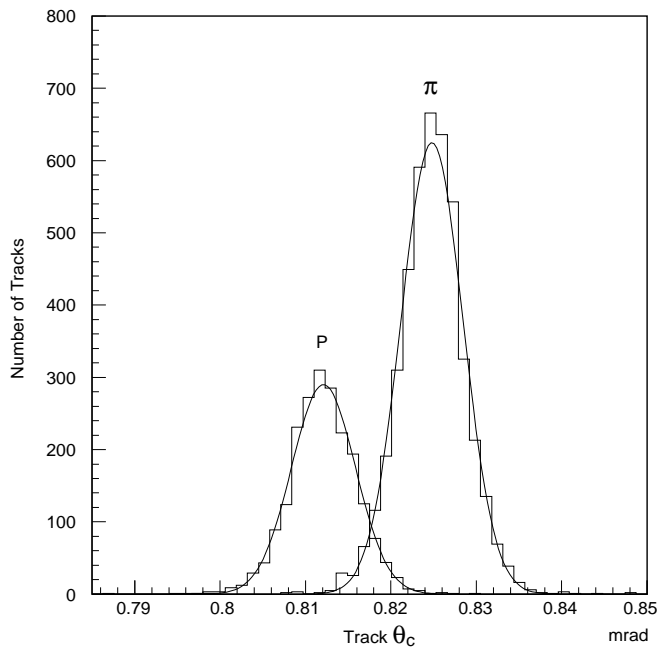
Figure 5: Cherenkov angle per track for pions and protons at 5.4 GeV/ c , with Z = 220 cm.
