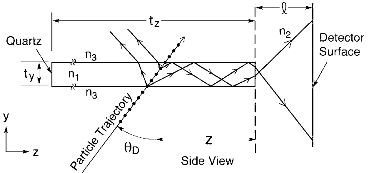
Figure 1: Imaging principle of the DIRC.
