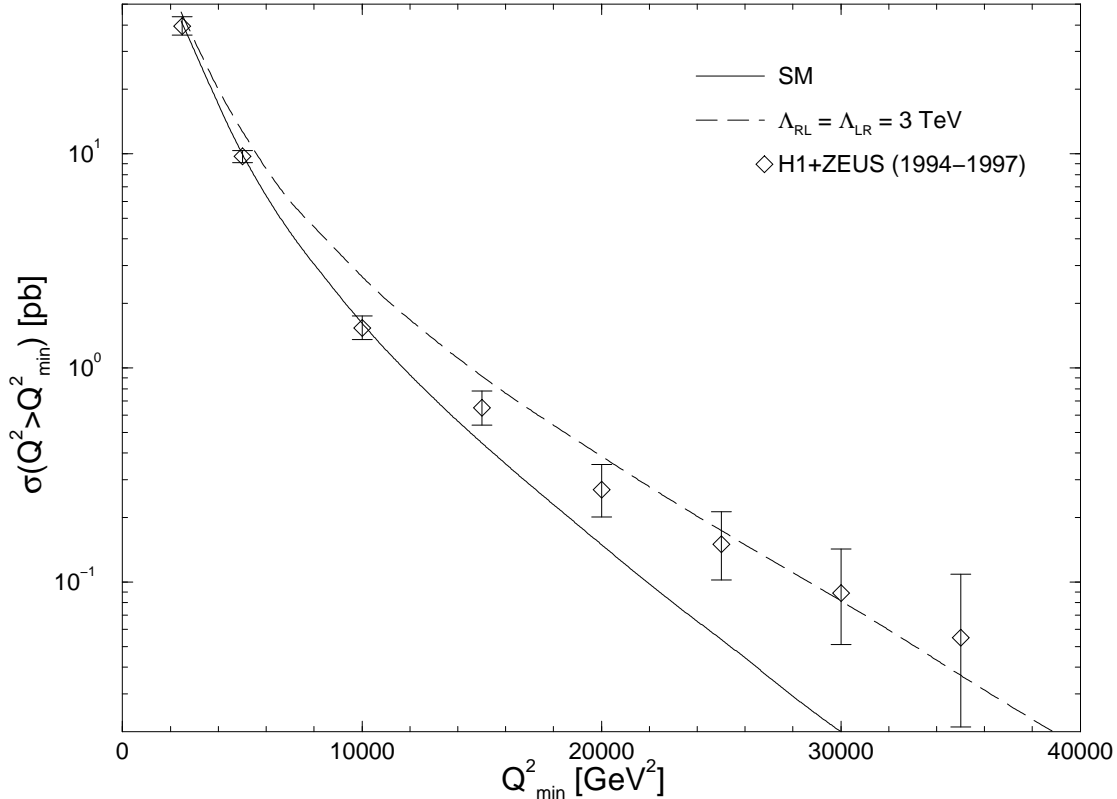
Figure 3: Cross-section for e^+p \rightarrow e^+X for Q^2 \geq Q_{min}^2 as a function of Q_{min}^2 in the Standard Model (solid line) and with an eu contact term with \Lambda_{RL} = \Lambda_{LR} = 3 \text{ TeV} . The combined experimental data from H1 and ZEUS are also shown.
