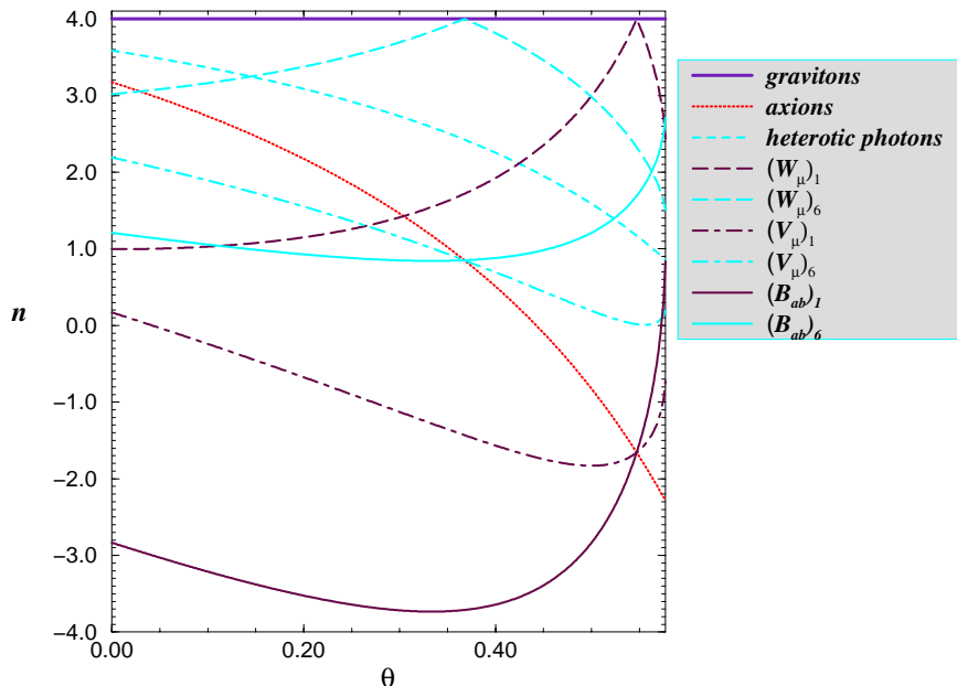
Figure 2: Same as Fig. 1 where, instead of fixing \theta , we fix \delta = -0.26 in the intermediate phase.
