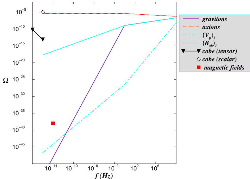
Figure 5: Some fluctuation spectra in the case of a string intermediate phase. The following choice of parameters was made: \zeta = 0.08 , \delta = -1/3 , f_1 \sim 10^{10} Hz, f_s \sim 8 \cdot 10^{-1} Hz, \varphi_s \sim -8 , \varphi_1 \sim -5 , T_{\text{eff}} = 2 \times 10^{18} GeV.
