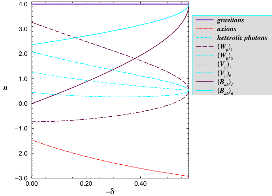
Figure 1: Spectral slopes for fluctuations that re-enter in the dual-dilaton phase when the latter is characterized by \theta = 1/\sqrt{3} (i.e. by constant moduli).
