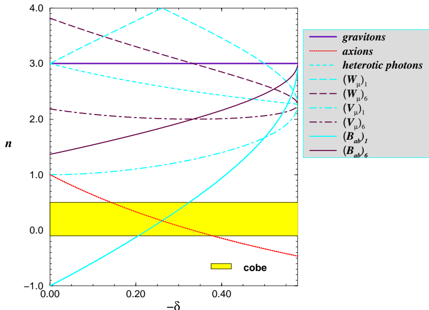
Figure 3: Spectral slopes for fluctuations that re-enter in the radiation phase. For comparison we also show the experimental constraint from COBE [20]: n + 1 = 1.2 \pm 0.3 .
