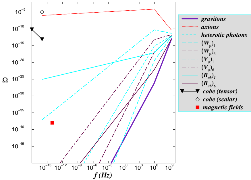
Figure 4: Spectrum for all the fluctuations considered in the case of a dual-dilaton intermediate phase, with the following choice: \delta = -0.3 , \theta = 1/\sqrt{3} , f_1 \sim 10^5 Hz, f_s \sim 10^9 Hz, \varphi_s \sim -23 , \varphi_1 \sim -11 , T_{\text{eff}} = 10^{15} GeV.
