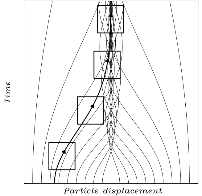
Fig. 1. The coarse-graining idea is exemplified in a schematic way based on a 2D tree-code simulation (Buchert 1996): the particles are attracted towards the pancake, a multi-stream region containing many streams (velocities) at a given Eulerian position. The coarsening cell follows initially a trajectory similar to that of individual particles. But as the cell moves into the pancake, the kinetic energy of the bulk motion is gradually transformed into internal kinetic energy, and its trajectory becomes qualitatively different from that of a particle.
