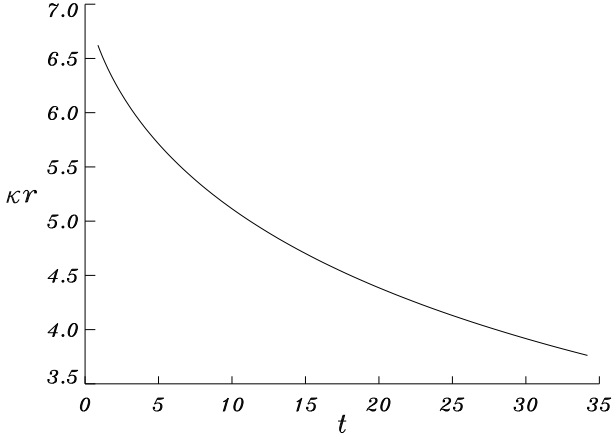
Fig. 1. \kappa r versus time in an undercritical FL background ( \Omega_0 < 1 ). \kappa r is measured in units of 10^{-3}(1 - \Omega_0)h^2 \text{ Gyr}^{-2} , and time is measured in units of \Omega_0(1 - \Omega_0)^{-3/2}h^{-1} \text{ Gyr} .
