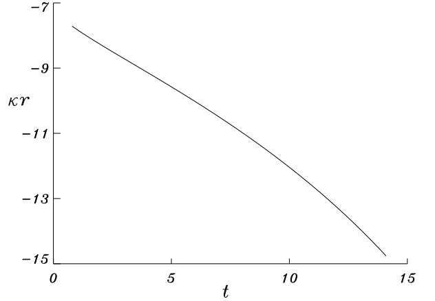
Fig. 2. \kappa r versus time in an overcritical FL background ( \Omega_0 > 1 ) up to the epoch of maximum expansion. \kappa r is measured in units of 10^{-3}(\Omega_0 - 1)h^2 \text{ Gyr}^{-2} , and time is measured in units of \Omega_0(\Omega_0 - 1)^{-3/2}h^{-1} \text{ Gyr} .
