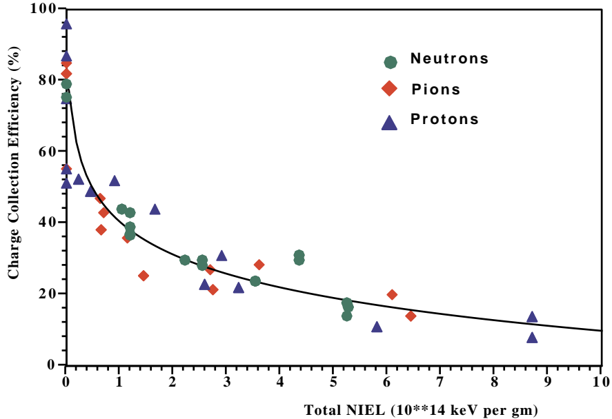
Figure 4: The charge collection efficiency as a function of total NIEL for ISIS neutrons, 300MeV/c pions and 24GeV/c protons for 200 \mu m thick SI-U LEC GaAs detectors
