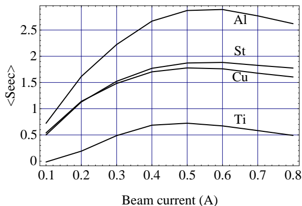
Figure: 5 \langle \text{sec} \rangle for different materials versus beam current for a 25 mm beam pipe
