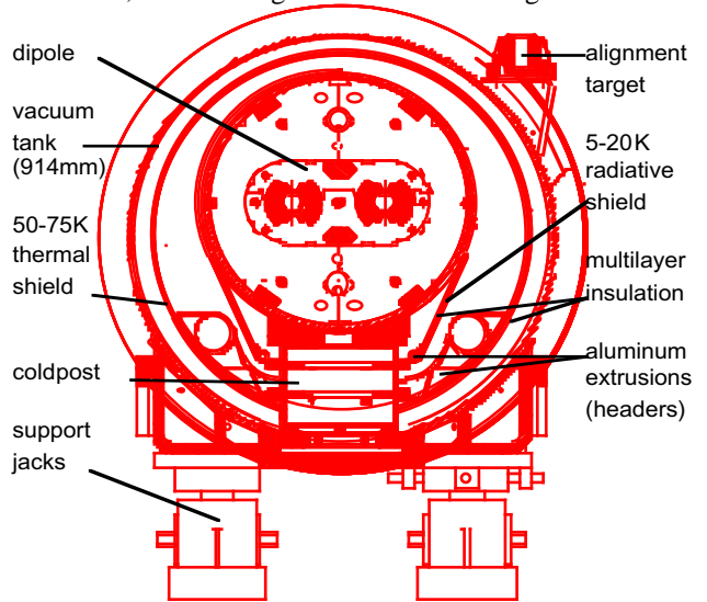
Figure 1: LHC Dipole Cryostat
