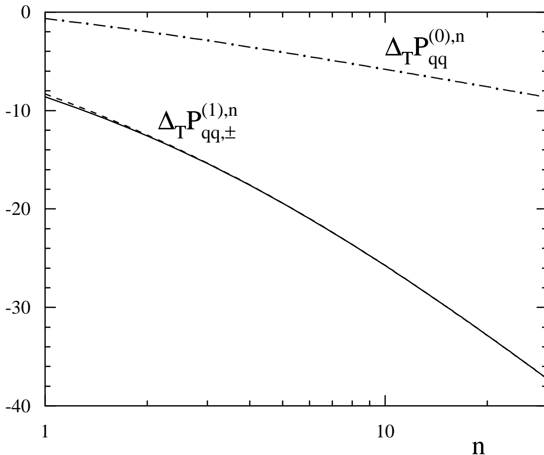
Figure 2: The Mellin- n moments of the NLO transversity splitting functions \Delta_T P_{qq,-}^{(1)} (solid line) and \Delta_T P_{qq,+}^{(1)} (dashed line) versus real n \geq 1 . For comparison the dash-dotted curve shows the LO result \Delta_T P_{qq}^{(0),n} .
