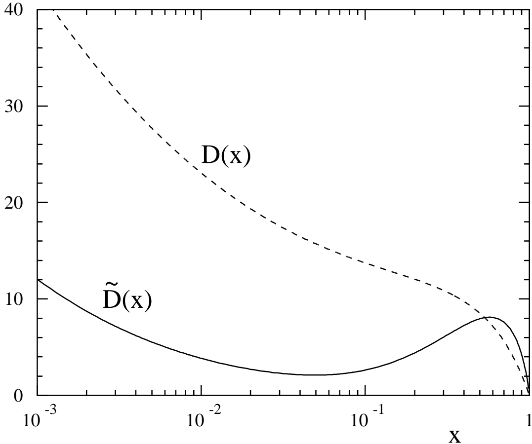
Figure 1: The functions \tilde{D}(x) , D(x) (see Eqs. (46),(49)) for f = 3 active flavours.
