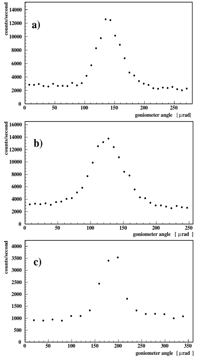
Figure 1: Angular scans, taken at different times to study reproducibility, Pb ions, 270 GeV/c per charge
