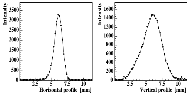
Figure 2: Horizontal and vertical profiles for optimum alignment, Pb ions, 270 GeV/c per charge
