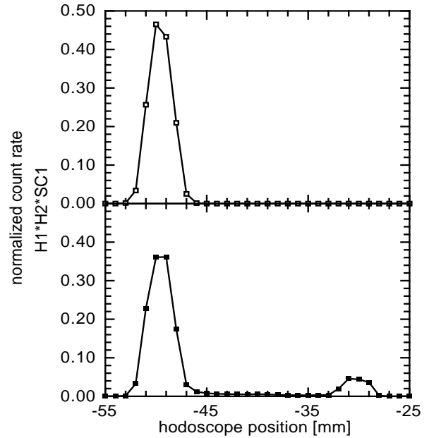
Figure 3: Vertical scan of the hodoscope (stepsize 1 mm) for the more divergent ('wide') Pb ion beam. For a non-aligned crystal (top), the straight beam peak is visible. Its intensity is reduced for the well-aligned crystal (bottom), and an additional peak of upwards deflected Pb ions is visible. (Note: The integrated number of counts is very similar in the two plots.)
