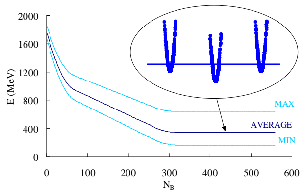
Figure 3. Energy profile along a drive beam pulse at the end of a drive linac section. The energy distribution within three subsequent bunches of the steady state part is also shown.
