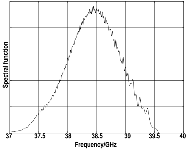
Figure: 5 Spectral function for cell/manifold coupled structure
