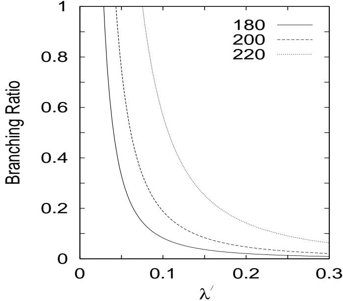
Figure 2: The R_p -violating branching fraction for the squark as a function of the coupling for three different values of the squark mass (marked, in GeV).
