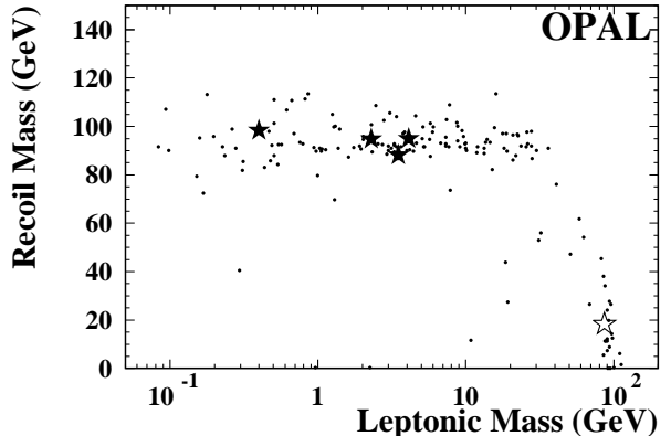
Figure 3: Scatter plot of the mass of the lepton pair and its recoil mass for the \mu\mu\text{qq} channel at 130-136 GeV, as observed by OPAL. The small points is the FERMISV expectation for the signal distribution. The four data events with large recoil mass are indicated by filled stars, whereas the open star represents a low recoil mass event. Summing all final states from all collabora-
