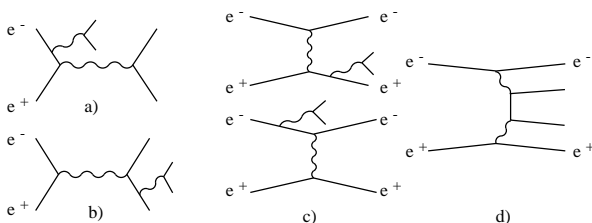
Figure 1: Feynman diagrams for four-fermion final states involving only neutral gauge boson exchange, represented by wiggly lines. The solid lines not labelled as e^\pm may be quarks, charged leptons, or neutrinos in case of Z exchange: a) “conversion”, b) “annihilation”, c) “bremsstrahlung”, and d) multiperipheral production.
