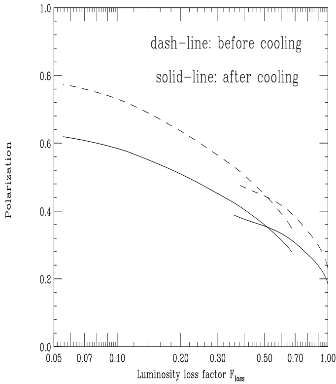
Figure 3: Polarization vs F_{\text{loss}} of muons accepted; the dashed line shows polarization as selected before cooling; the solid line gives polarization after cooling.
