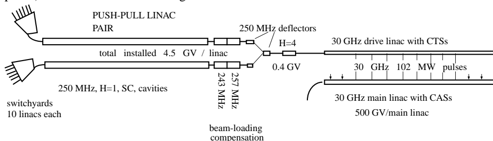
Fig. 1. Generation of one drive beam upstream of one drive linac.
