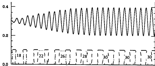
Fig. 5. H = 4 excitation by the prefill train pairs (upper trace). The drive train pairs (bottom trace) are also shown. Only a small fraction (600J, 0.7%) of one drive beam energy (90 kJ) is used for energizing. Furthermore it is taken from the first trains which are underdecelerated in the drive linac. The voltage obtained is 6.1 MV/m.
