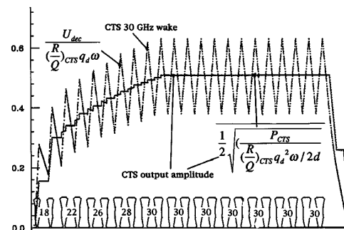
Fig. 2. Computer optimized bunchlet numbers, relative intensities, normalized 30 GHz CTS wake amplitudes (dashed, linear variations of \pm 23\% ) and the normalized CTS output amplitude.
