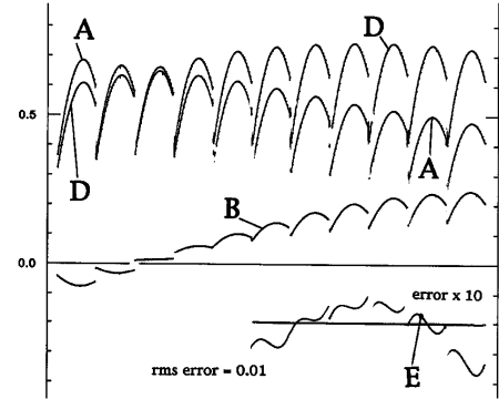
Fig. 4. Decrease of normalized (with respect to the sum of all installed cavity peak voltages) accelerating H = 1 voltage due to beam-loading over 11 trains of bunchlets (upper full trace A). Curve B shows the compensating voltage obtained as a fast beat between the 2 groups of compensating cavities with 29% of the total installed voltage and frequencies of 243 and 257 MHz. Curve D is the sum of A and B. Curve E is the error with respect to constant amplitude during the flat top. Only the successive short phase intervals (of 90^\circ ) populated by the bunchlets of each train are shown, whereas the remaining unpopulated 270^\circ in each of the 11 periods have been cut out . The error with respect to the ideal H = 1 oscillation is 0.01 rms.
