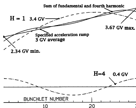
Fig. 3. Acceleration ramp synthesis.
