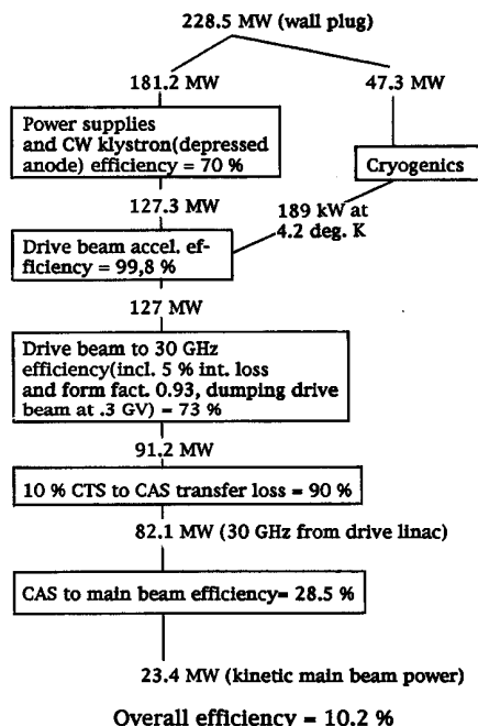
Fig. 6. Wall plug to main beam efficiency.
