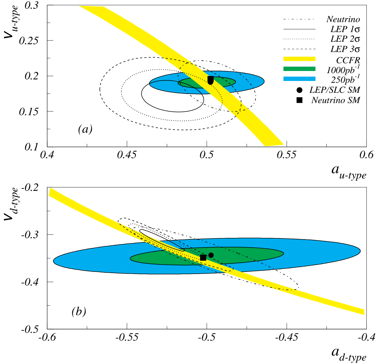
Figure 2: Summary of measurements of u-type (a) and d-type (b) quark couplings to the Z^0 . The results of a measurement at HERA are shown as the shaded ellipses. The outer ellipse shows the result which would be obtained with 250 \text{ pb}^{-1} divided equally between the four lepton beam charge/polarization combinations, the inner ellipse shows the result which would be obtained with 1000 \text{ pb}^{-1} equally divided. Fits for the couplings of the u (d) quarks were performed with the d (u) quark couplings fixed at their SM values. The open ellipse drawn with a dash-dotted line shows the one standard deviation ( 1\sigma ) contour obtained in a fit of the four chiral couplings of the u and d quarks to a compilation of neutrino DIS data. The solid, dotted and dashed ellipses show the 1, 2 and 3 \sigma limits of the combined LEP/SLD results for the c and b quark couplings. The shaded band shows the result obtained by the CCFR collaboration from the ratio of NC and CC cross sections projected onto the quark coupling plane. In the case of the CCFR the couplings of the u (d) quarks are obtained with the d (u) quark couplings fixed at their SM values. SM coupling values including radiative corrections appropriate for comparison with e^+e^- (circle) and neutrino (square) measurements are also shown.
