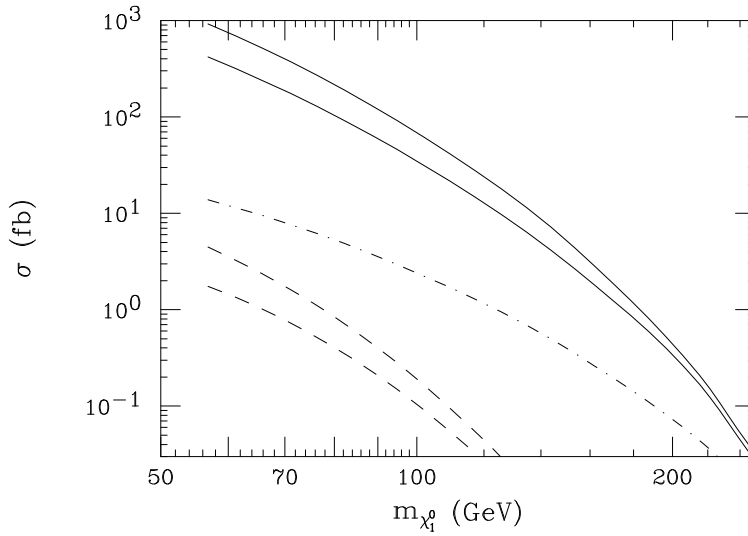
Figure 19: Production cross sections (fb) for p\bar{p} initial state to the final states \chi_1^\pm\chi_2^0 (upper solid line), \chi_1^+\chi_1^- (lower solid line), \tilde{l}_R^+\tilde{l}_R^- (dot-dashed line), \tilde{\nu}_L\tilde{l}_L^\pm (upper dashed line), and \tilde{l}_L^+\tilde{l}_L^- (lower dashed line). Lepton flavors are not summed. The center of mass energy is 2 TeV, \text{sgn}(\mu) = +1 , and \Lambda = M .
