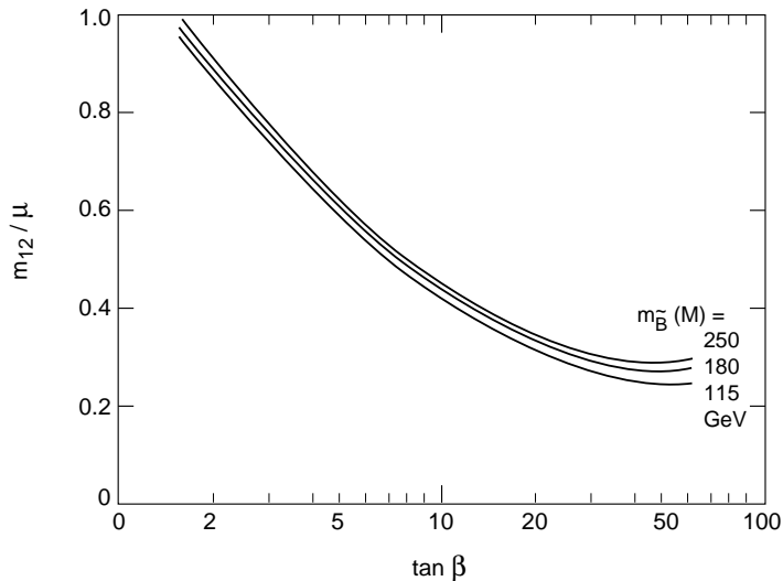
Figure 6: The ratio m_{12}/\mu as a function of \tan \beta imposed by electroweak symmetry breaking for m_{\tilde{B}}(M) = 115, 180, 250 GeV and \Lambda = M .
