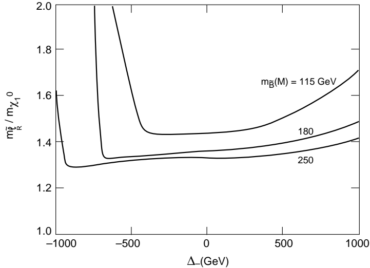
Figure 16: The ratio m_{\tilde{l}_R^0}/m_{\chi_1^0} as a function of \Delta_- at the messenger scale for m_{\tilde{B}}(M) = 115, 180, 250 GeV, \tan\beta = 3 , \text{sgn}(\mu) = +1 , and \Lambda = M .
