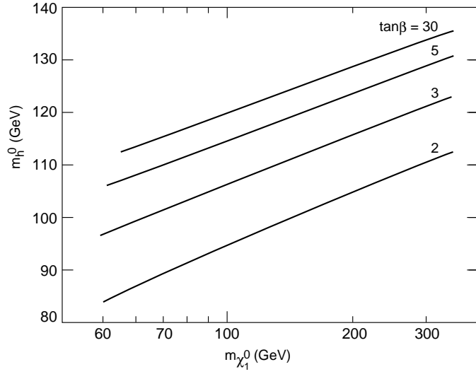
Figure 11: The lightest Higgs mass, m_{h^0} , as a function of the lightest neutralino mass, m_{\chi_1^0} , for \tan\beta = 2, 3, 5, 30 , and \Lambda = M .
