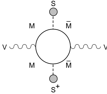
Figure 1: One-loop messenger sector supergraph which gives rise to visible sector gaugino masses.
