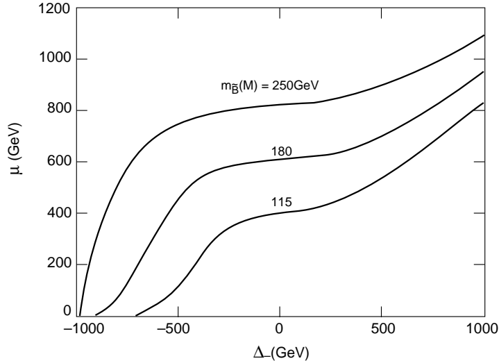
Figure 15: The relation between the low scale |\mu| parameter and \Delta_- \equiv \text{sgn}(\Delta_-^2(M))(|\Delta_-^2(M)|)^{1/2} at the messenger scale imposed by electroweak symmetry breaking for \Delta_+(M) = 0 , m_{\tilde{B}}(M) = 115, 180, 250 , GeV \tan \beta = 3 , and \Lambda = M .
