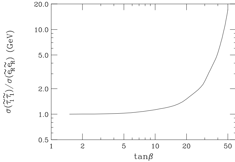
Figure 21: The ratio \sigma(p\bar{p} \rightarrow \tilde{\tau}_1^+ \tilde{\tau}_1^-) / \sigma(p\bar{p} \rightarrow \tilde{e}_R^+ \tilde{e}_R^-) as a function of \tan\beta for m_{\tilde{B}}(M) = 115 GeV and \Lambda = M . The center of mass energy is 2 TeV.
