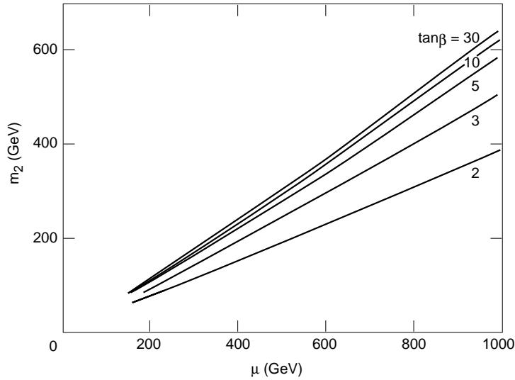
Figure 5: The relation between m_2 and |\mu| imposed by electroweak symmetry breaking with MGM boundary conditions for \tan\beta = 2, 3, 5, 10, 30 , and \Lambda = M .
