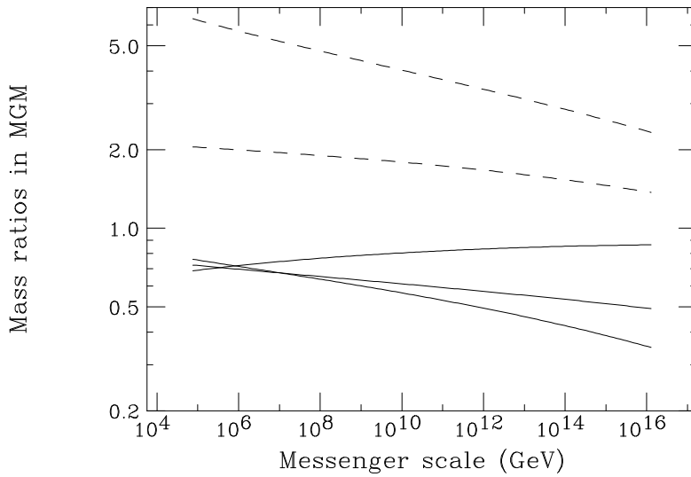
Figure 13: Ratios of \overline{DR} mass parameters with MGM boundary conditions as a function of the messenger scale: m_{\tilde{q}_R}/m_{\tilde{l}_R} (upper dashed line), m_{\tilde{l}_L}/m_{\tilde{l}_R} (lower dashed line), m_3/m_{\tilde{q}_R} (upper solid line), m_2/m_{\tilde{l}_L} (middle solid line), and m_1/m_{\tilde{l}_R} (lower solid line).
