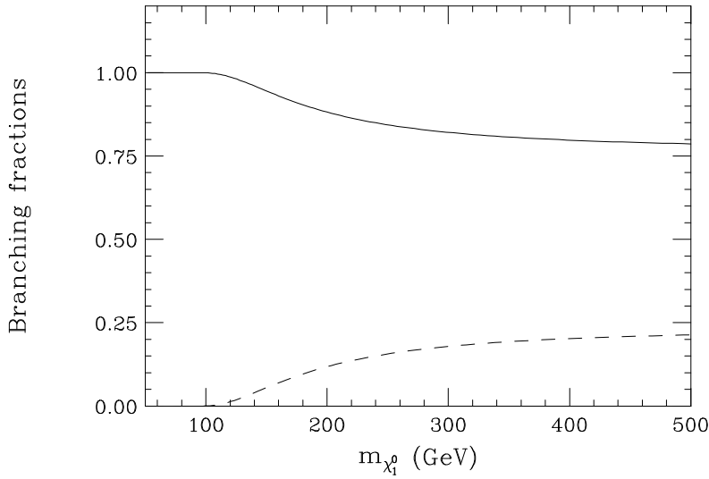
Figure 20: The branching ratios for \chi_1^0 \rightarrow \gamma + G (solid line) and \chi_1^0 \rightarrow Z^0 + G (dashed line) as a function of m_{\chi_1^0} for \Lambda = M .
