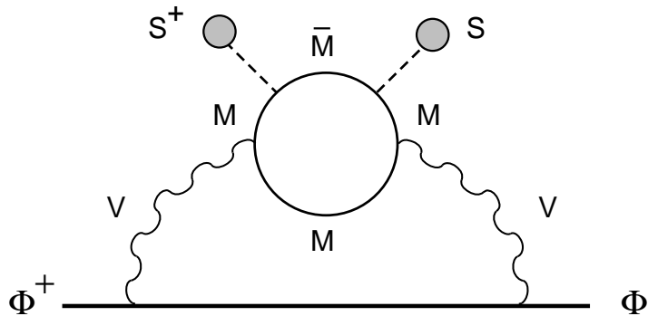
Figure 2: Two-loop messenger sector supergraph which gives rise to visible sector scalar masses. The one-loop subgraph gives rise to visible sector gaugino wave function renormalization. Other graphs related by gauge invariance are not shown.
