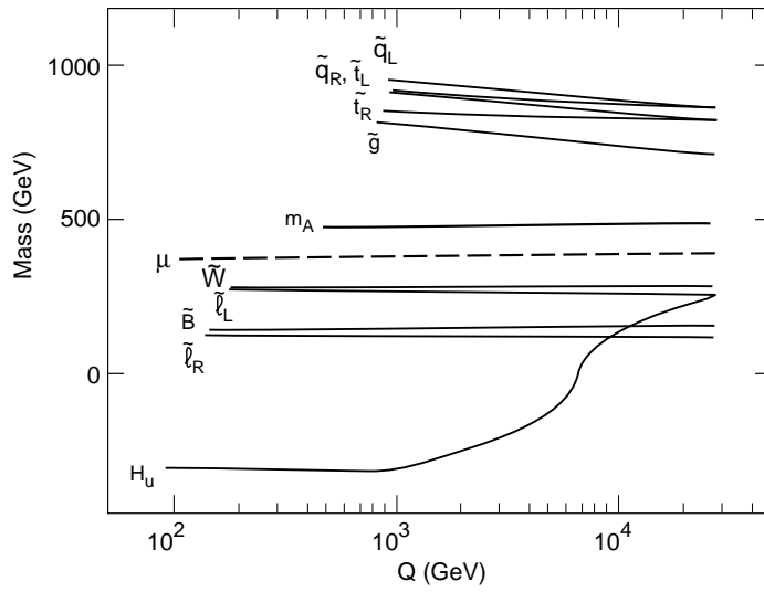
Figure 14: Renormalization group evolution of the \overline{\text{DR}} mass parameters with boundary conditions of the two generation messenger sector. The messenger scale is M = 54 TeV, \Lambda = M , m_{\tilde{B}}(M) = 163 GeV, and \tan \beta = 3 .
