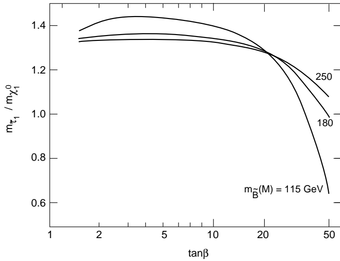
Figure 8: The ratio m_{\tilde{\tau}_1}/m_{\chi_1^0} as a function of \tan\beta for m_{\tilde{B}}(M) = 115, 180, 250 GeV. For large \tan\beta the \tilde{\tau}_1 becomes the lightest standard model superpartner.
