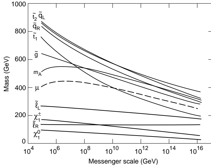
Figure 12: The physical spectrum as a function of the messenger scale for m_{\tilde{B}}(M) = 115 GeV and \tan \beta = 3 .
