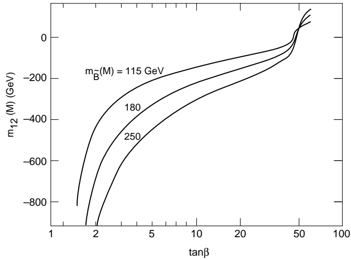
Figure 17: The relation between m_{12}(M) and \tan\beta imposed by electroweak symmetry breaking for m_{\tilde{B}}(M) = 115, 180, 250 GeV, and \Lambda = M .
