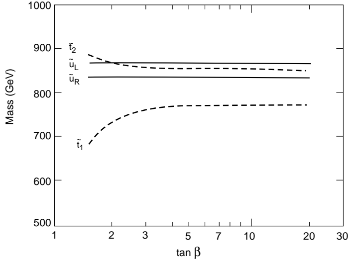
Figure 9: Squark spectrum as a function of \tan\beta for m_{\tilde{B}}(M) = 115 GeV and \Lambda = M .
