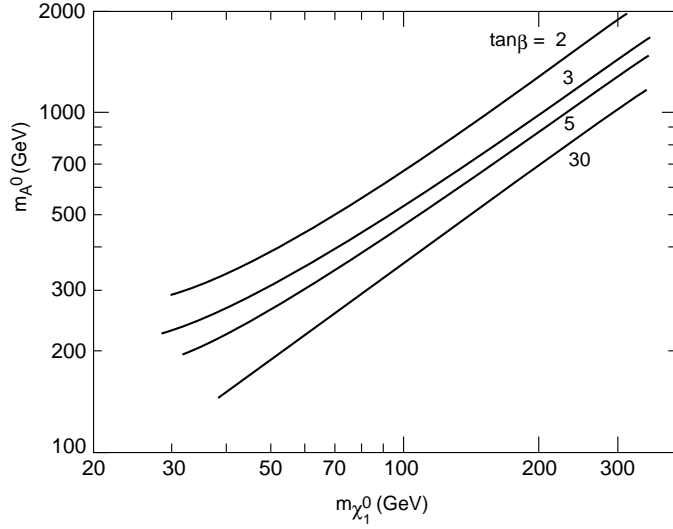
Figure 10: The pseudo-scalar Higgs mass, m_{A^0} , as a function of the lightest neutralino mass, m_{\chi_1^0} , for \tan\beta = 2, 3, 5, 30 , and \Lambda = M .
