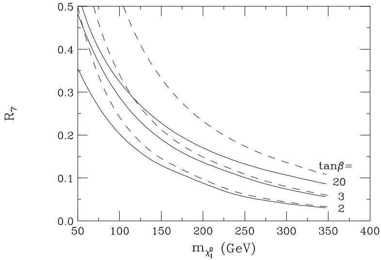
Figure 18: The parameter R_7 \equiv C_7^{\text{MSSM}}(m_{W^\pm})/C_7^{\text{SM}}(m_{W^\pm}) - 1 as a function of the lightest neutralino mass, m_{\chi_1^0} , for \tan\beta = 2, 3, 20 , and \Lambda = M . The solid lines are for \mu > 0 and the dashed lines for \mu < 0 .
