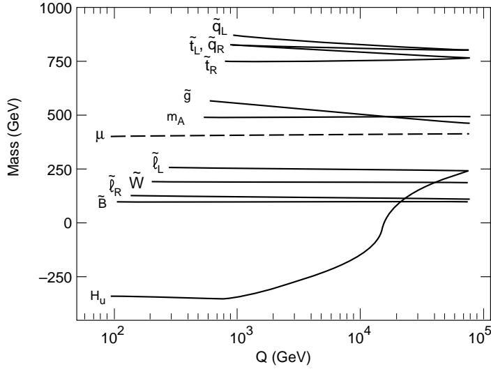
Figure 4: Renormalization group evolution of the \overline{\text{DR}} mass parameters with MGM boundary conditions. The messenger scale is M = 76 \text{ TeV} , m_{\tilde{B}}(M) = 115 \text{ GeV} , \tan \beta = 3 , \text{sgn}(\mu) = +1 , and m_t^{\text{pole}} = 175 \text{ GeV} . The masses are plotted as m \equiv \text{sgn}(m)(|m|)^{1/2} .
