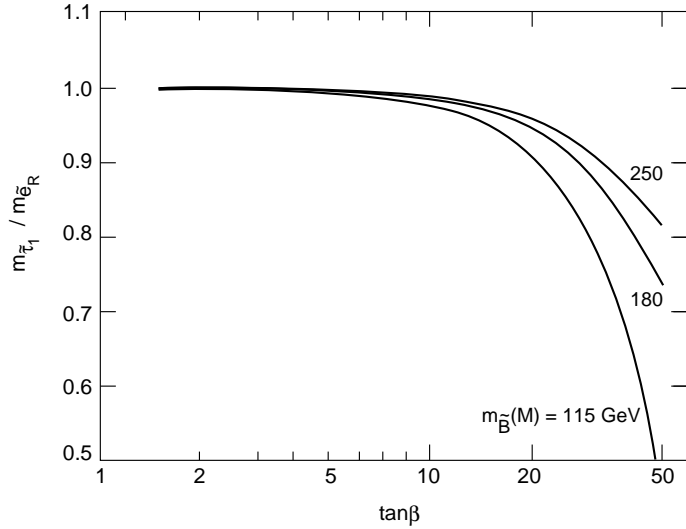
Figure 7: The ratio m_{\tilde{\tau}_1}/m_{\tilde{e}_R} as a function of \tan\beta for m_{\tilde{B}}(M) = 115, 180, 250 GeV, and \Lambda = M .
