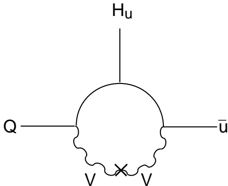
Figure 3: One-loop visible sector supergraph which contains both logarithmic and finite contributions to visible sector A -terms. The cross on the visible sector gaugino line represents the gaugino mass insertion shown in Fig. 1.
