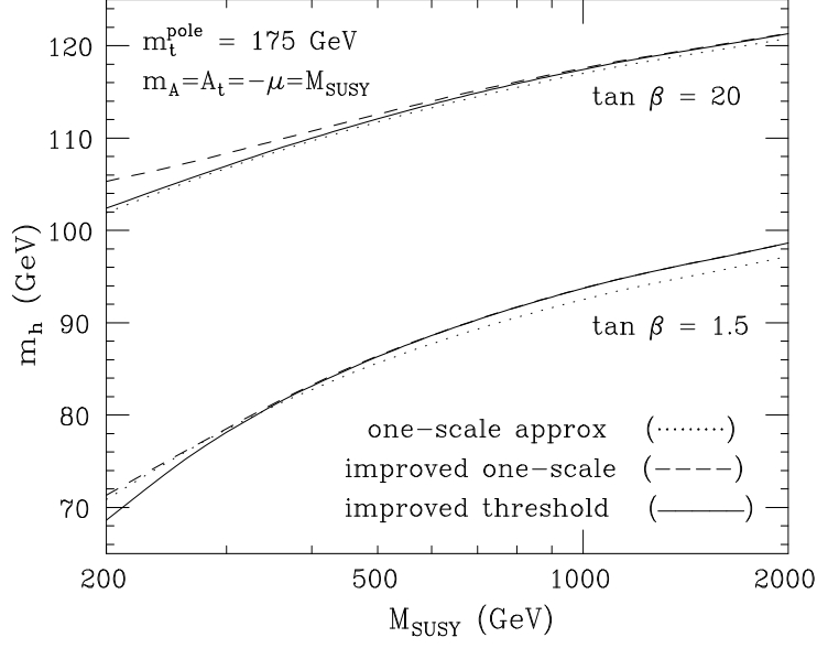
Fig. 10. The radiatively corrected light RG-improved CP-even Higgs mass is plotted as a function of M_{\text{SUSY}} for m_{A^0} = A_t = -\mu = M_Q = M_U = M_D = M_{\text{SUSY}} . Two choices of \tan\beta = 1.5 and \tan\beta = 20 are shown. The results are based on the analytic approximation given in eq. (3.25). In the one-scale approximation (dotted line), the distinction between M_{\text{SUSY}} and third generation squark masses are neglected. In addition, radiative corrections proportional to \ln(m_{A^0}^2/m_Z^2) and the non-leading log term proportional to m_t^2 are neglected, as discussed below eq. (A.5). These approximations were also made in the graphs of all previous figures. In the improved one-scale approximation (dashed line), the latter two neglected terms are included. In addition, the factors of M_{\text{SUSY}}^2 in the argument of the leading logs of Appendix A are replaced by the appropriate product of third generation squark masses, as described below eq. (A.6). In the improved threshold approximation, we include the corrections of Appendix C with the replacement of M_Q , M_U , and M_D by the corresponding third generation squark masses as described below eq. (C.11).
