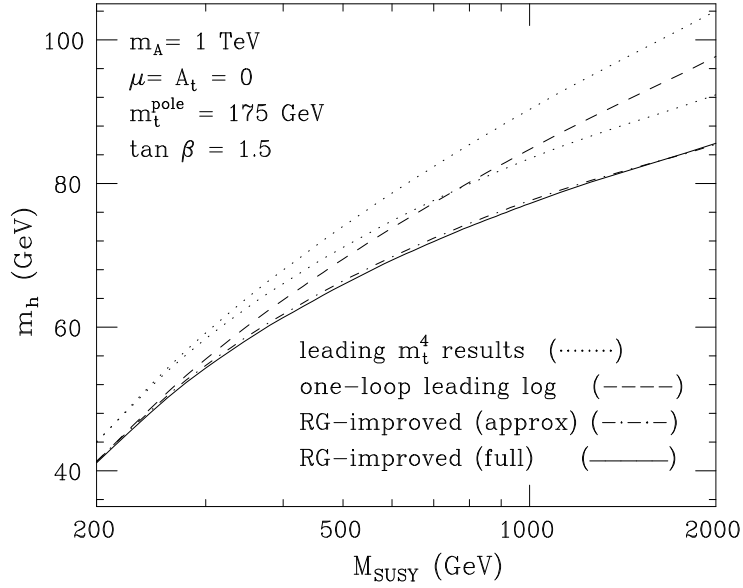
Fig. 2. The radiatively corrected light CP-even Higgs mass is plotted as a function of M_{\text{SUSY}} for \tan \beta = 1.5 and m_{A^0} = 1 TeV. See the caption to Fig. 1.
