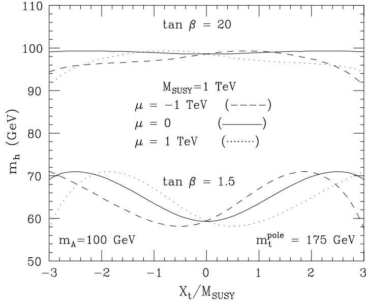
Fig. 7. The radiatively corrected, RG-improved light CP-even Higgs mass is plotted as a function of X_t/M_{\text{SUSY}} for M_{\text{SUSY}} = 1 TeV and m_{A^0} = 100 GeV. See the caption to Fig. 6.
