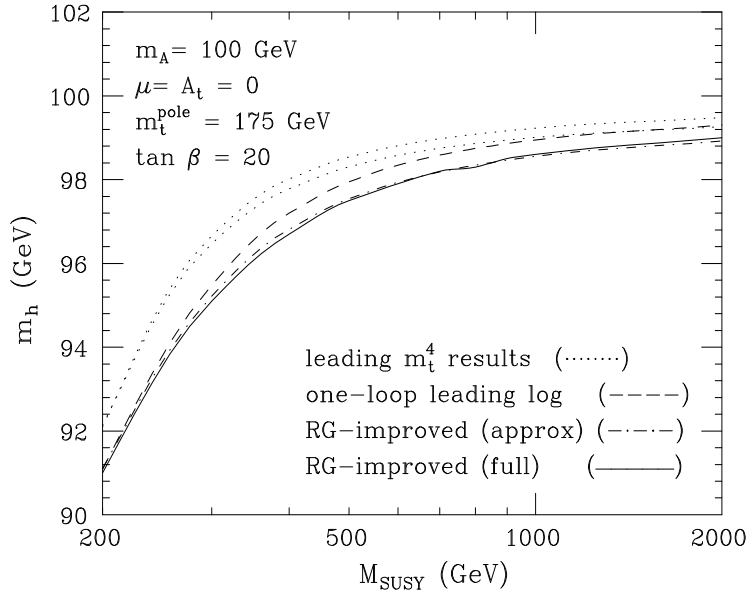
Fig. 3. The radiatively corrected light CP-even Higgs mass is plotted as a function of M_{\text{SUSY}} for \tan \beta = 20 and m_{A^0} = 100 GeV. See the caption to Fig. 1.
